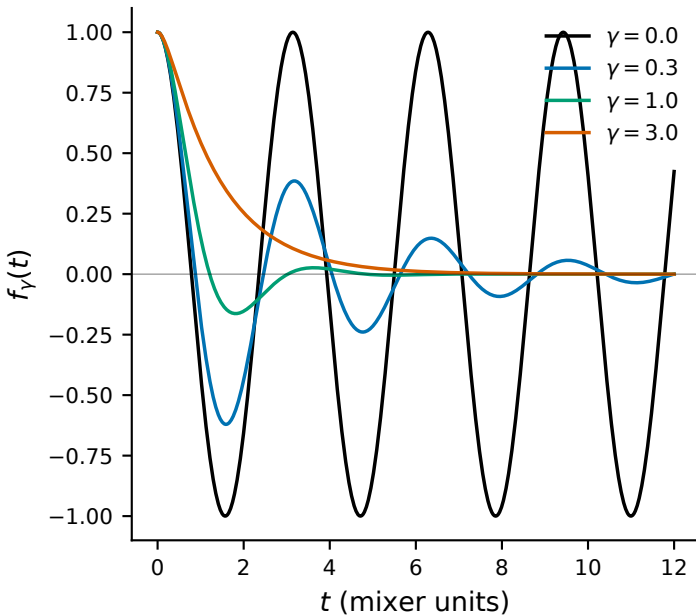
(a) telegraph f_\gamma(t)
