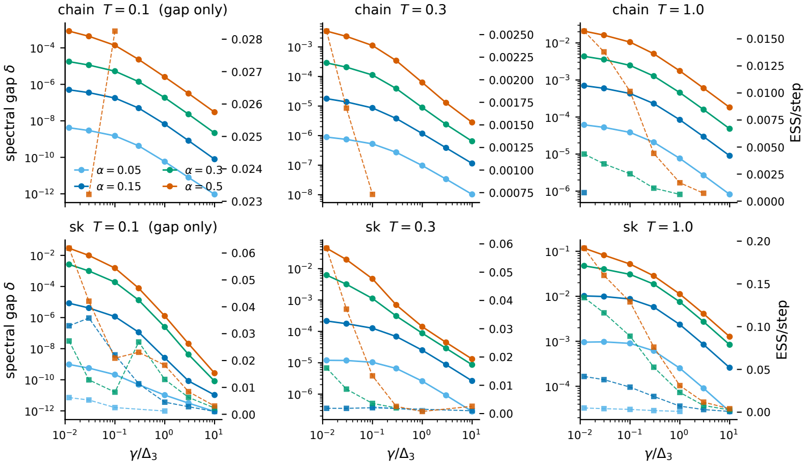
T=0.1 cells are gap-only (ESS unmeasurable at 50k steps, R-hat-gated).
