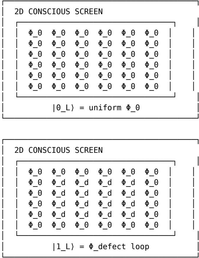
Figure 10: Logical qubit encoding in global \Phi -patterns
