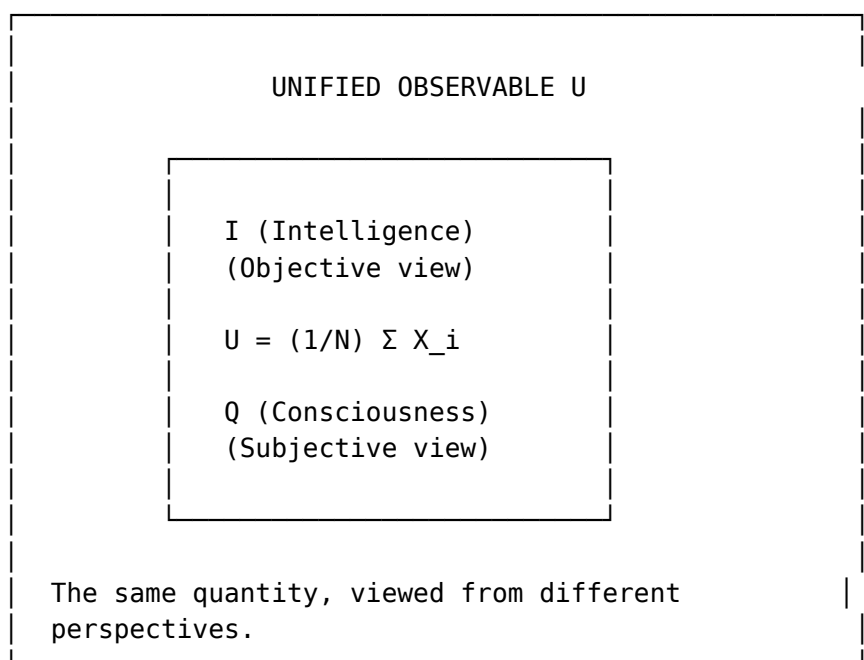
Figure 26: The unified observable \mathcal{U} as the dual-aspect monism of the HNN
