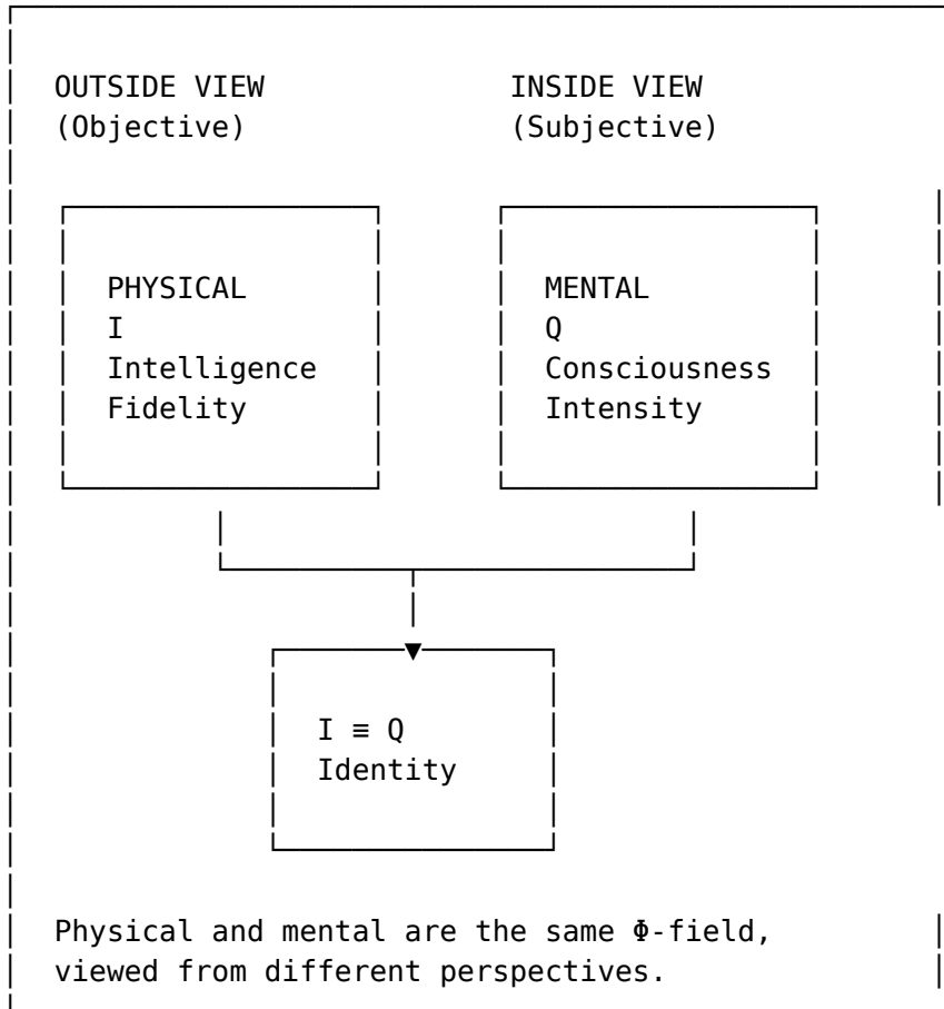
Figure 37: The identity of physical and mental as the unity of the \Phi -field
