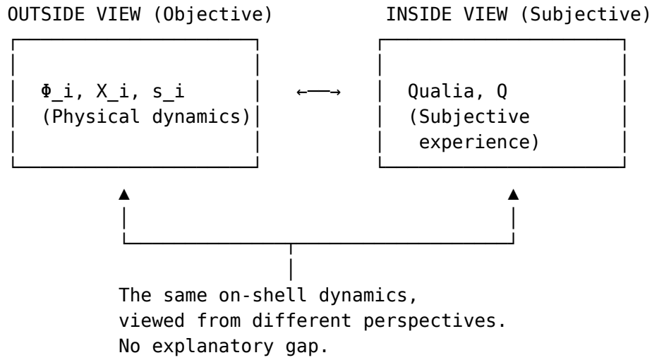
Figure 18: The dissolution of the hard problem
