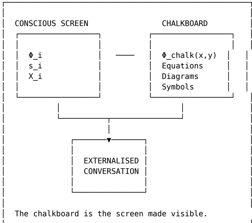
Figure 71: The chalkboard as the external screen
