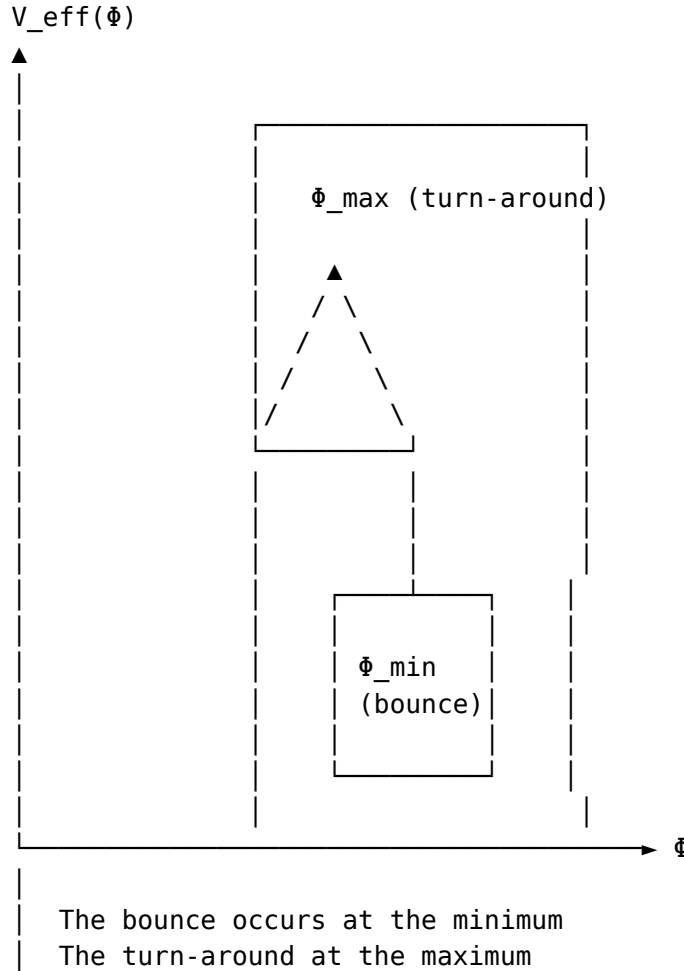
Figure 56: The effective potential and the bounce
