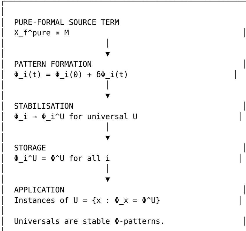
Figure 42: Universals as stable \Phi -configurations
