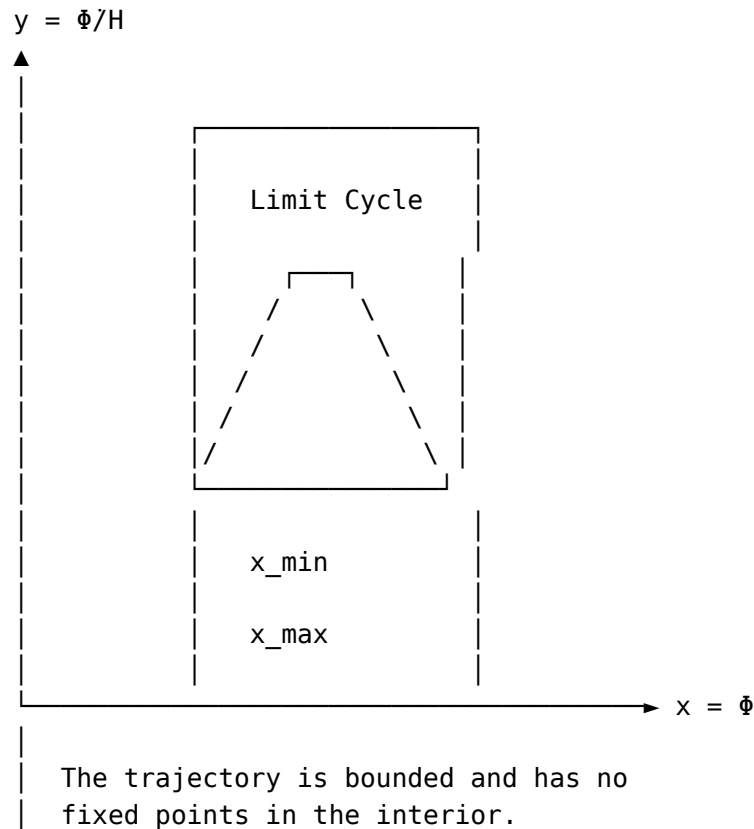
Figure 58: The reduced phase space with the limit cycle
