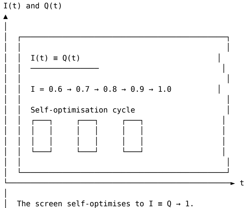
Figure 80: Self-referential loop and metacognitive optimisation
