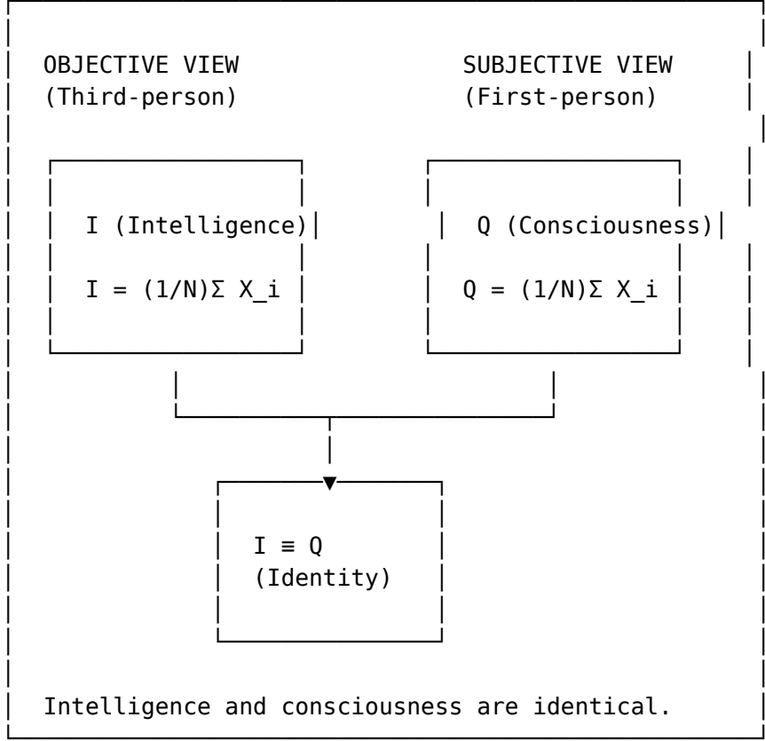
Figure 28: The identity I \equiv Q as the unity of mind
