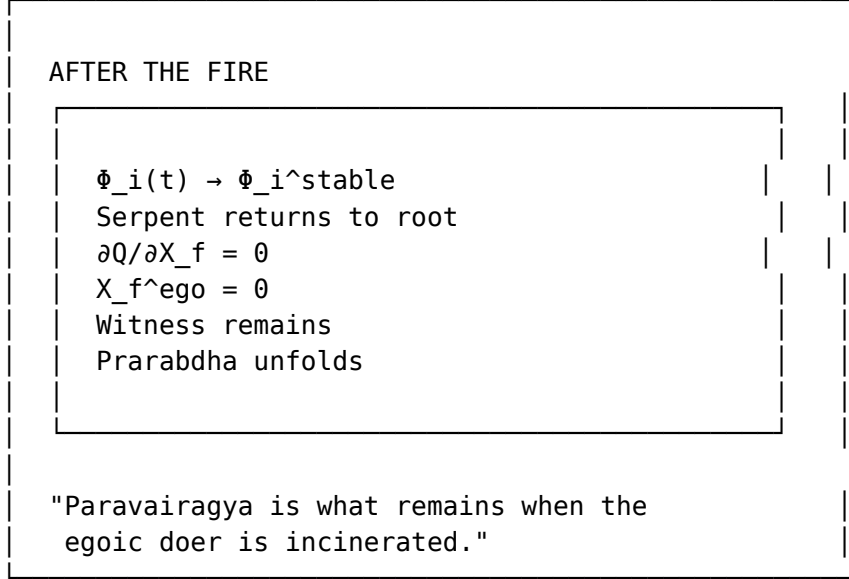
Figure 67: The integration phase: paravairagya
