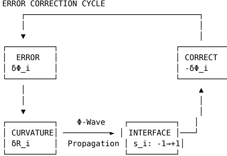
Figure 4: The holographic error correction cycle
