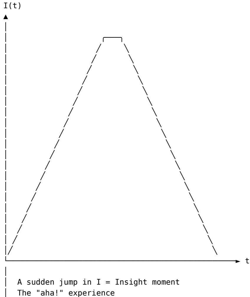
Figure 24: Insight as a sudden jump in intelligence fidelity
