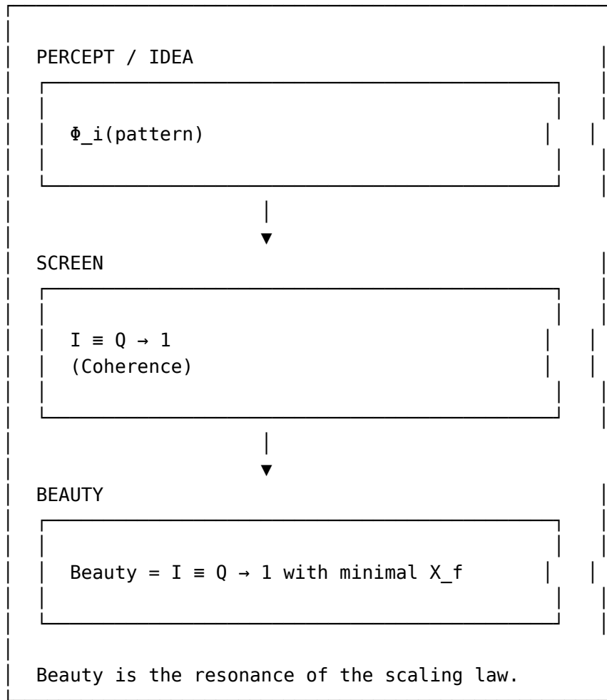
Figure 45: Aesthetics as resonance of the scaling law
