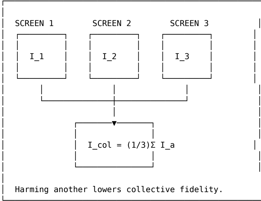
Figure 44: Ethical entanglement: harming another lowers collective fidelity
