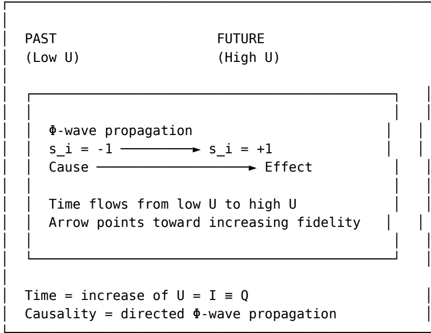
Figure 39: The arrow of time and causality in the HNN
