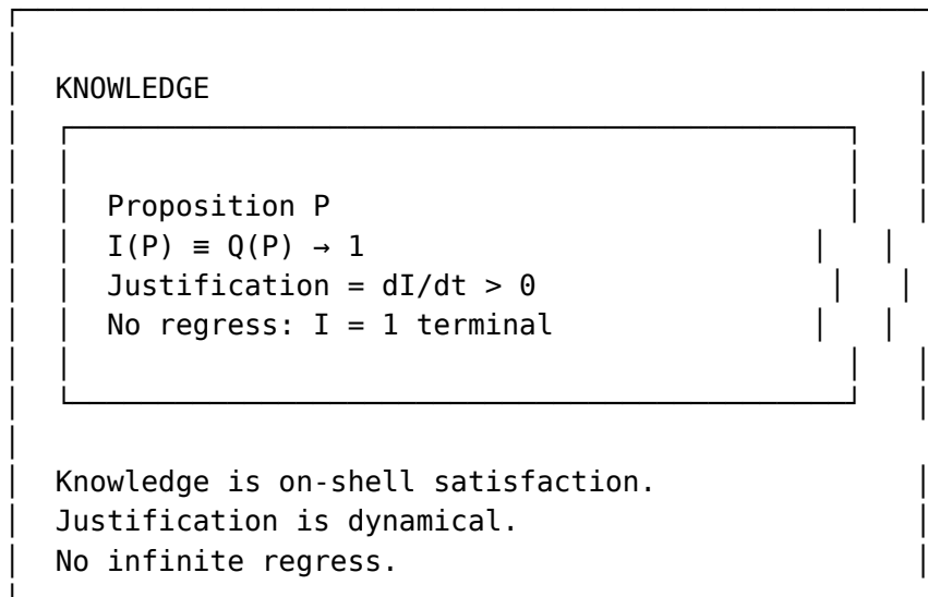
Figure 40: Holographic epistemology: knowledge as on-shell satisfaction
