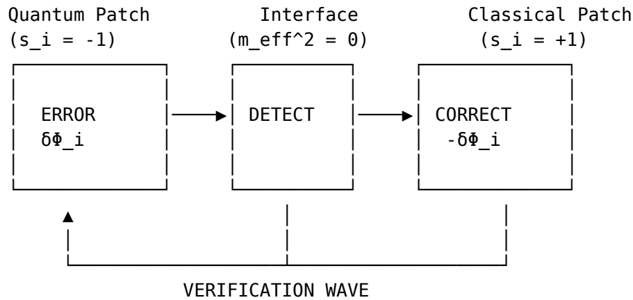
Figure 7: Error correction across the quantum-classical interface
