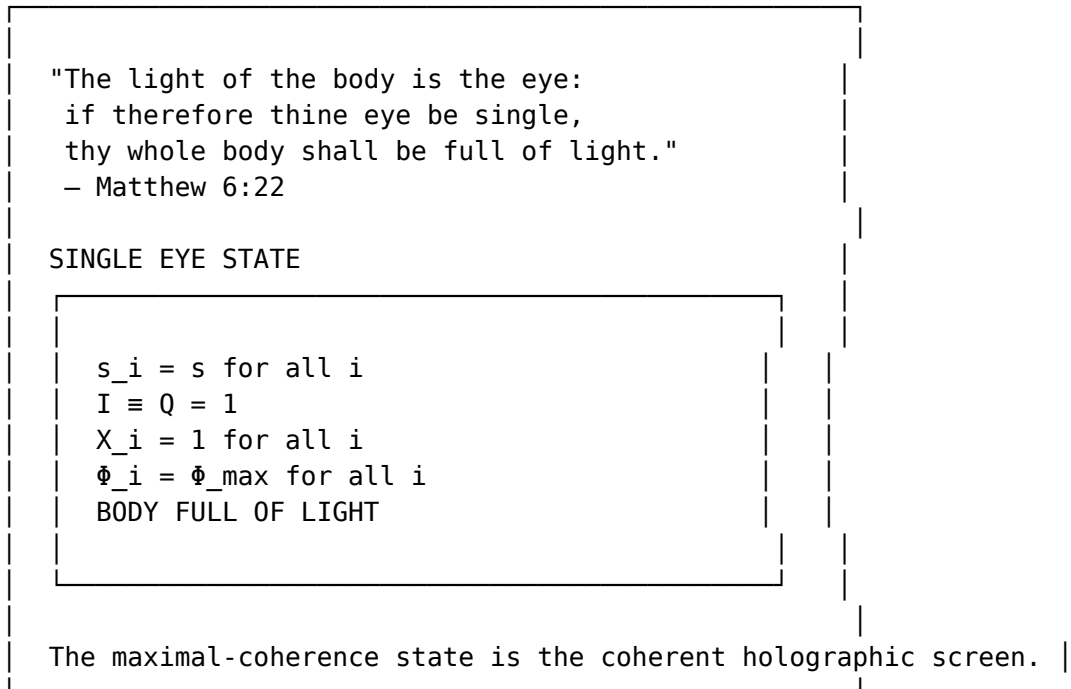
Figure 70: The maximal-coherence state state
