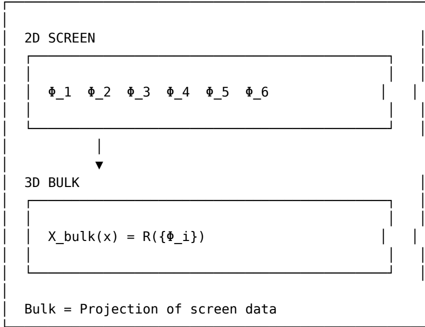
Figure 34: Holographic projection from the 2D screen to the bulk
