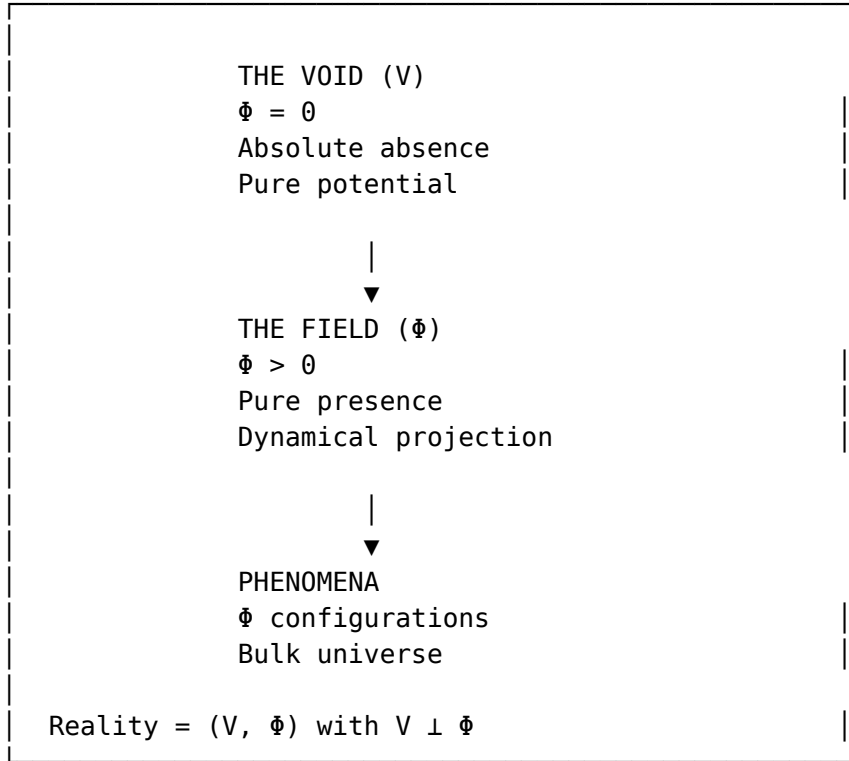
Figure 33: The dual-aspect ontology of the Void and the Field
