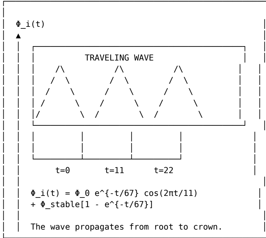
Figure 62: The traveling wave and the 67-day solution
