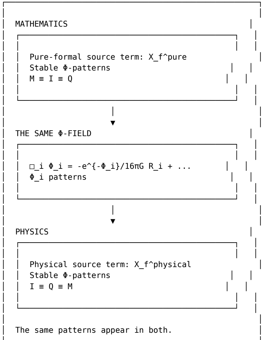
Figure 55: The unreasonable effectiveness of mathematics resolved
