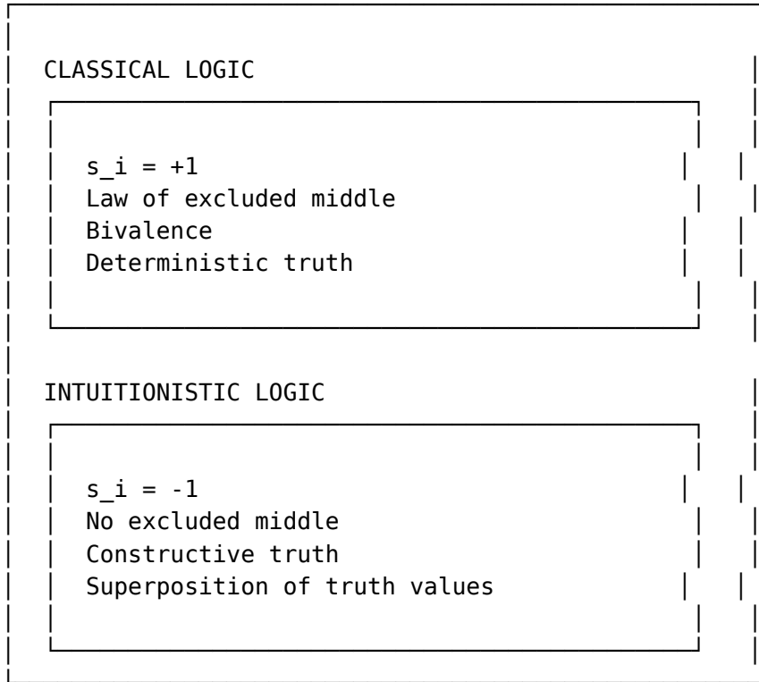
Figure 47: Logic from dynamic regime partitioning
