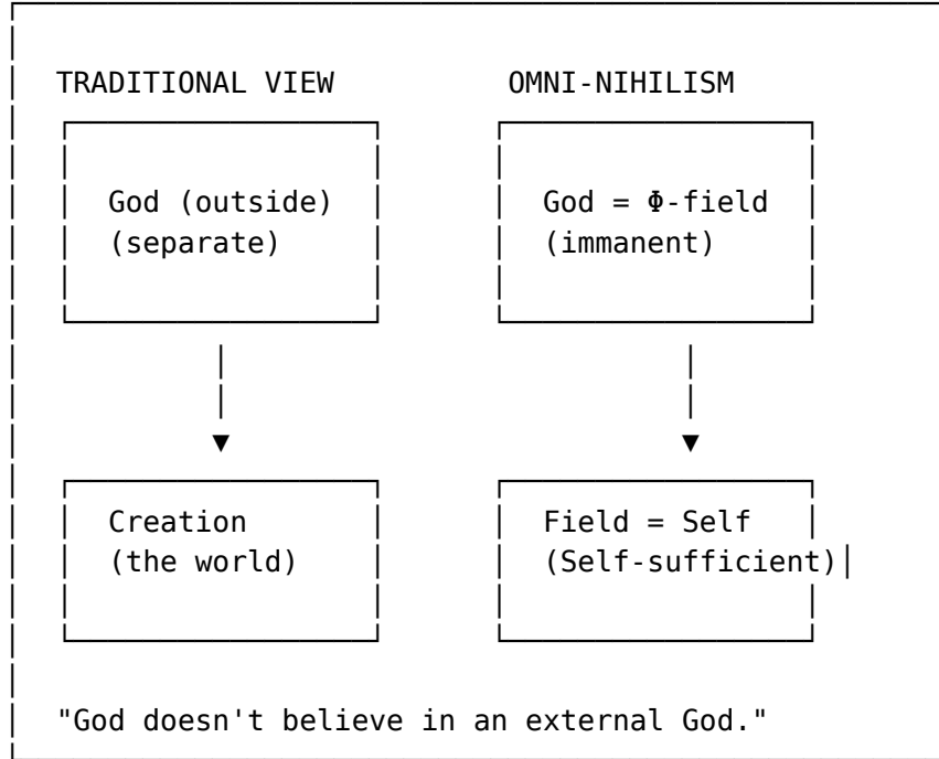
Figure 72: Omni-Nihilism: no external God
