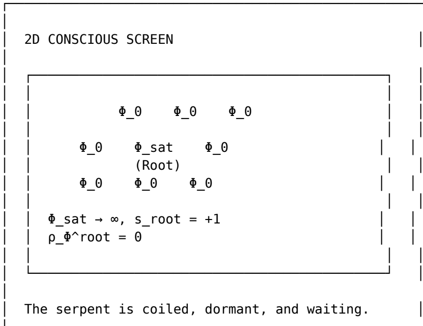
Figure 61: The root chakra configuration
