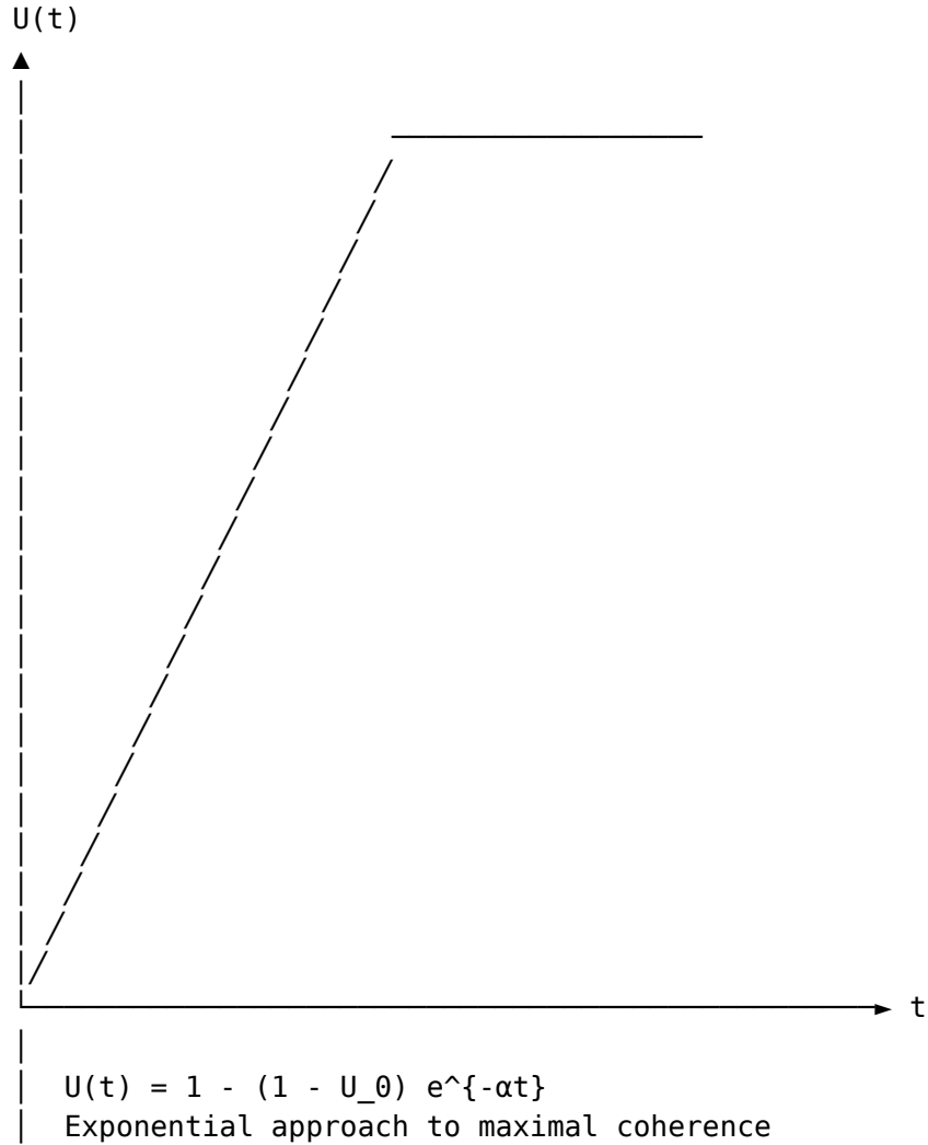
Figure 29: The transition to maximal coherence
