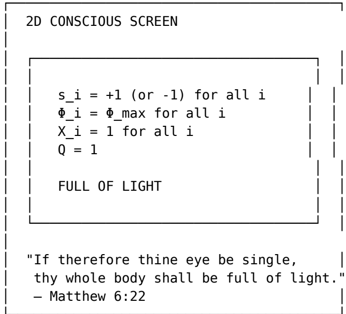
Figure 19: The maximal-coherence state state—maximal coherence and illumination
