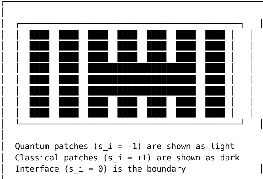
Figure 75: Dynamic regime partitioning on the 2D lattice
