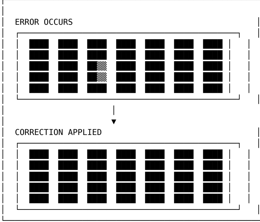
Figure 77: Error correction on the holographic lattice
