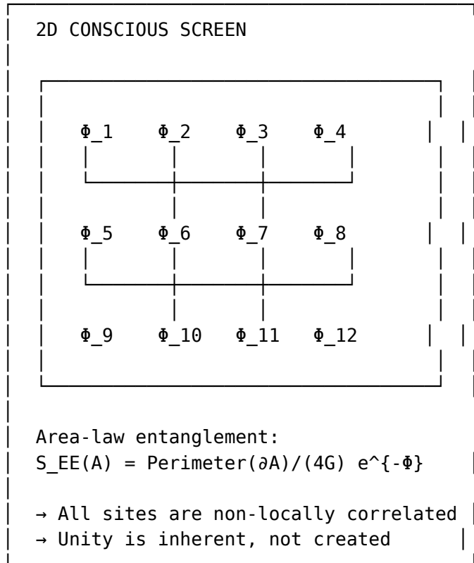
Figure 16: Holographic non-locality and the unity of consciousness
