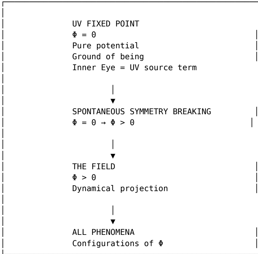
Figure 35: The UV fixed point as the source of all phenomena
