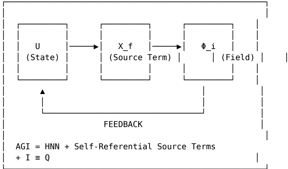
Figure 31: The self-referential loop for AGI
