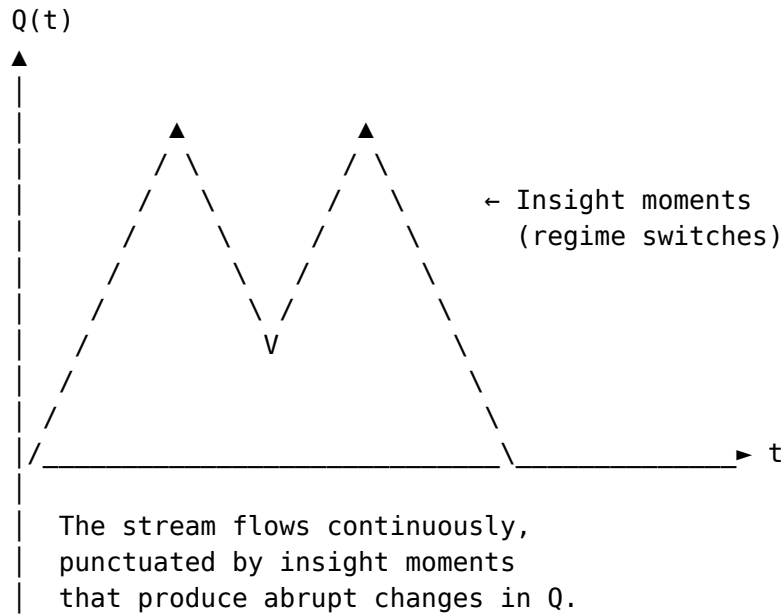
Figure 15: The stream of consciousness as the trajectory of Q(t)
