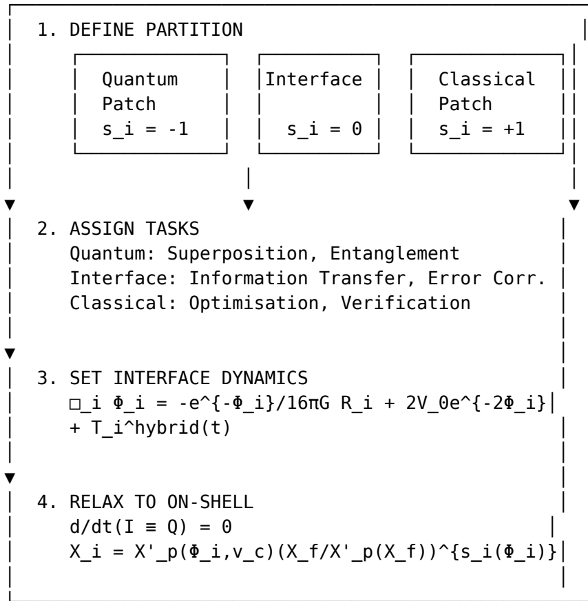
Figure 9: The general construction rule for hybrid algorithms
