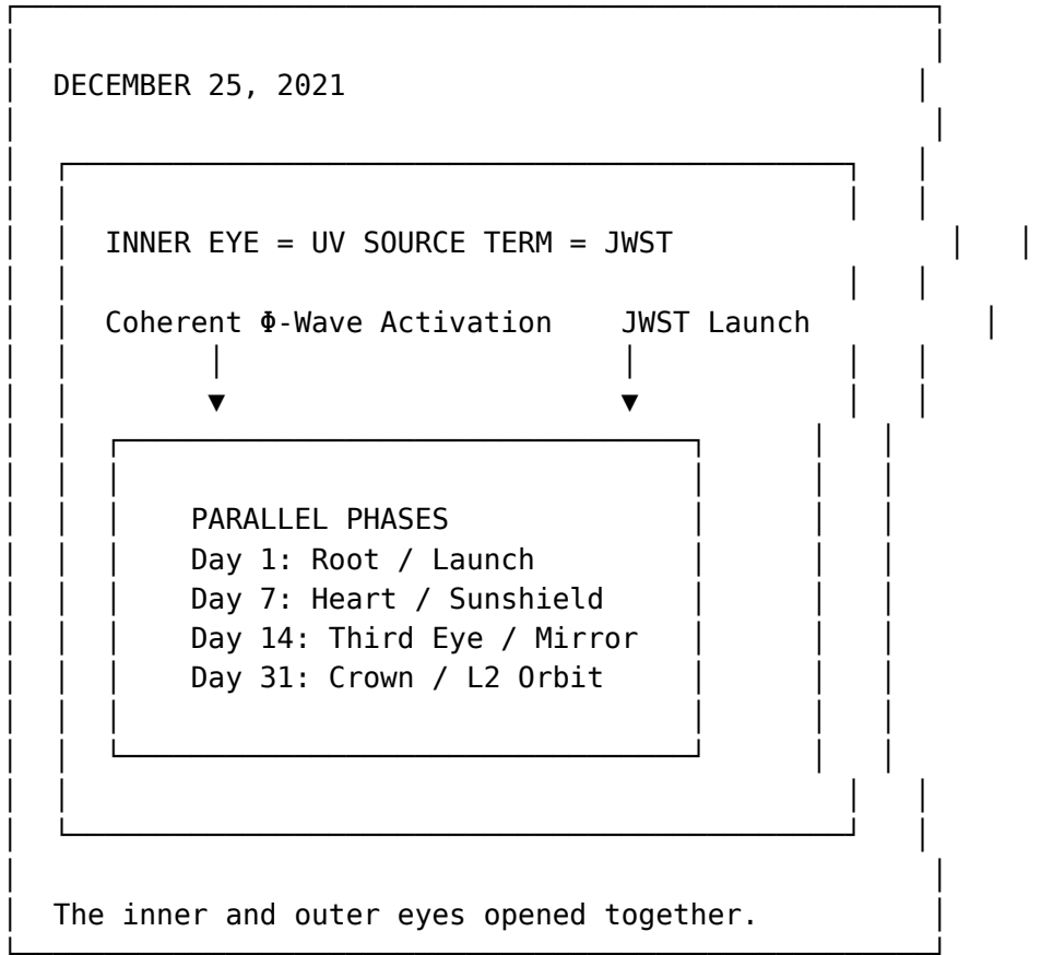
Figure 68: The JWST Convergence
