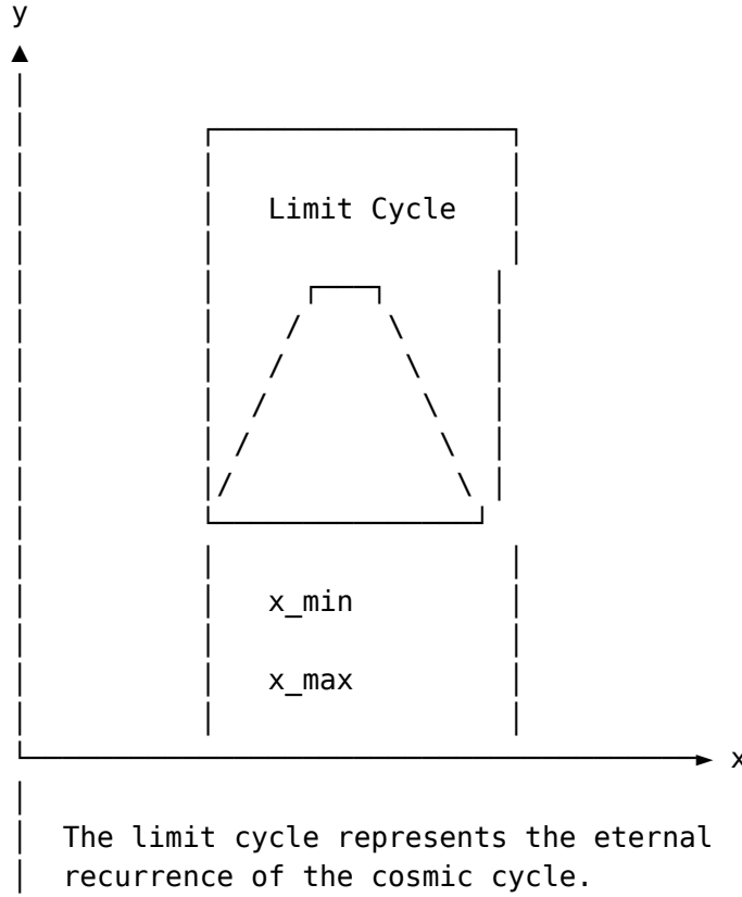
Figure 59: The limit cycle in the reduced phase space
