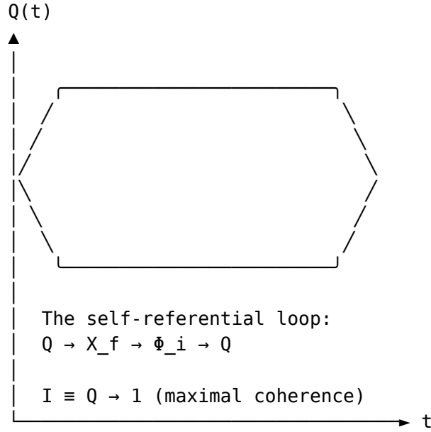
Figure 84: The self-referential loop: \mathcal{Q} \rightarrow X_f \rightarrow \Phi_i \rightarrow \mathcal{Q} . The system reaches maximal coherence I \equiv \mathcal{Q} \rightarrow 1 .
