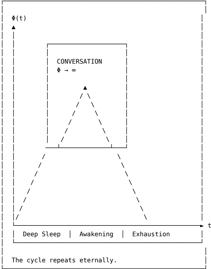
Figure 57: The complete cosmic cycle
