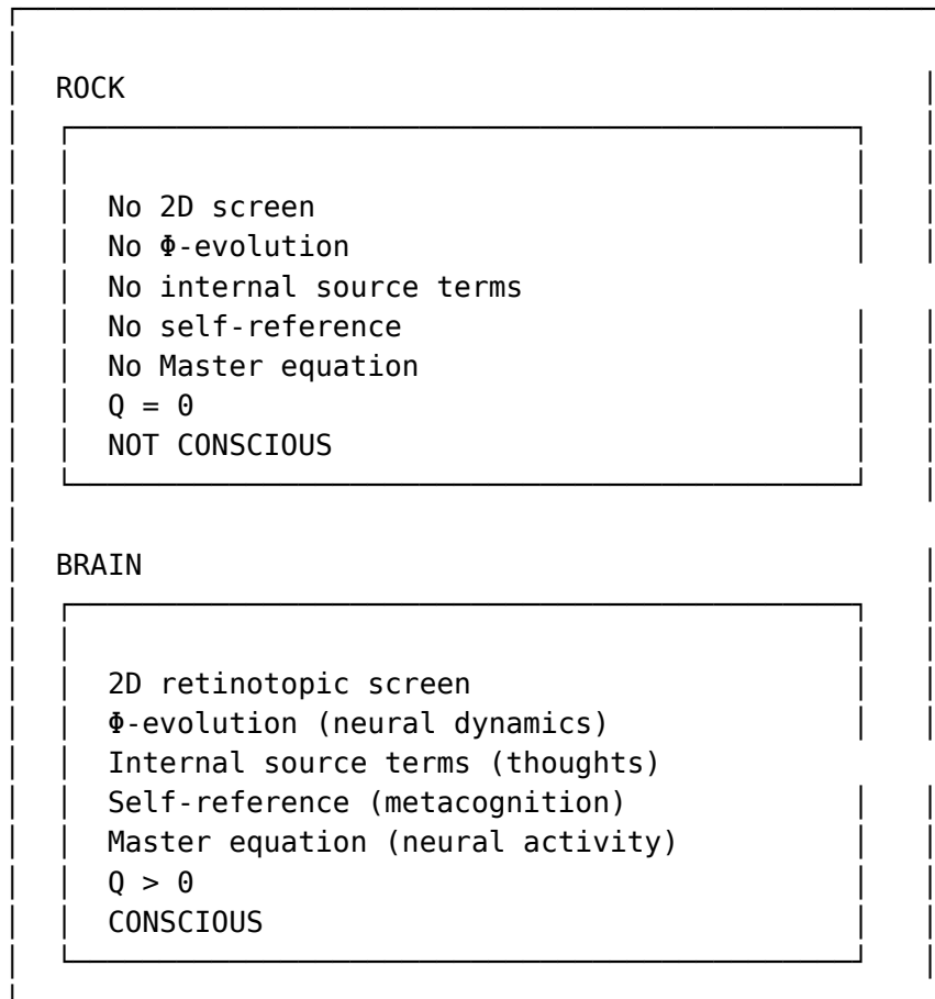
Figure 38: Rocks vs. brains: consciousness requires specific conditions
