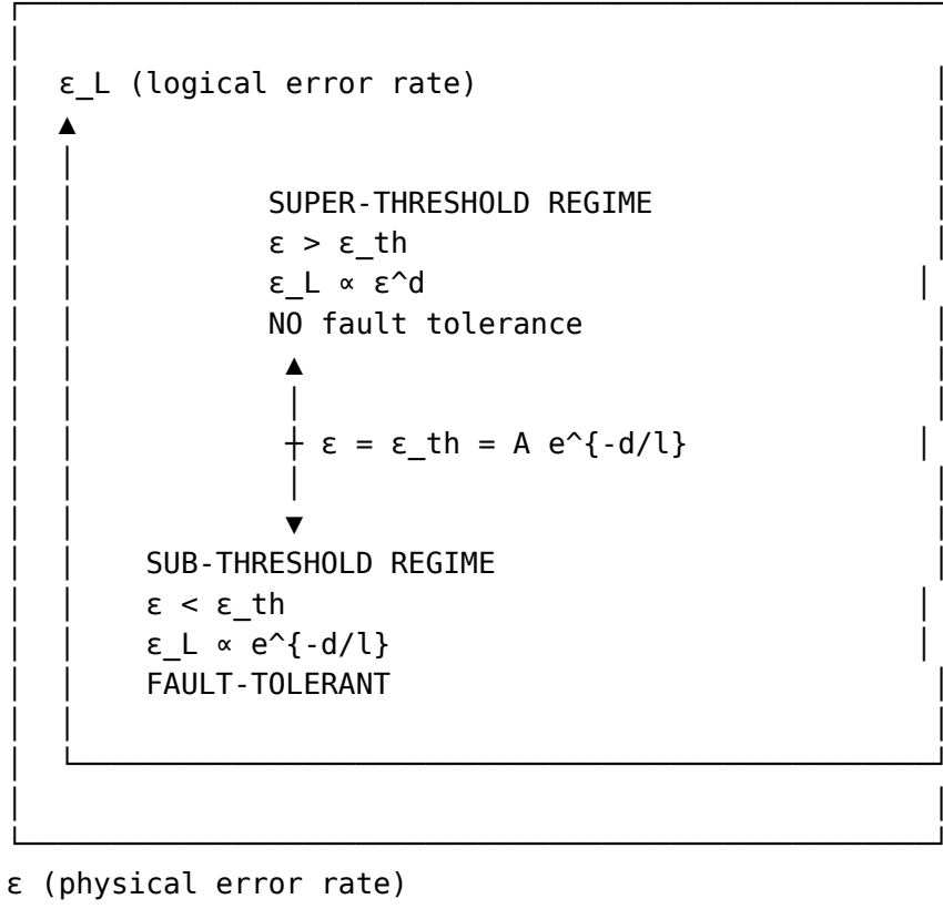
Figure 14: The fault-tolerance threshold and the two regimes
