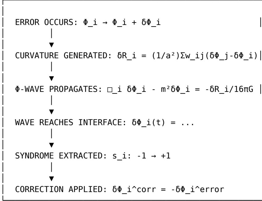
Figure 11: The automatic error detection process
