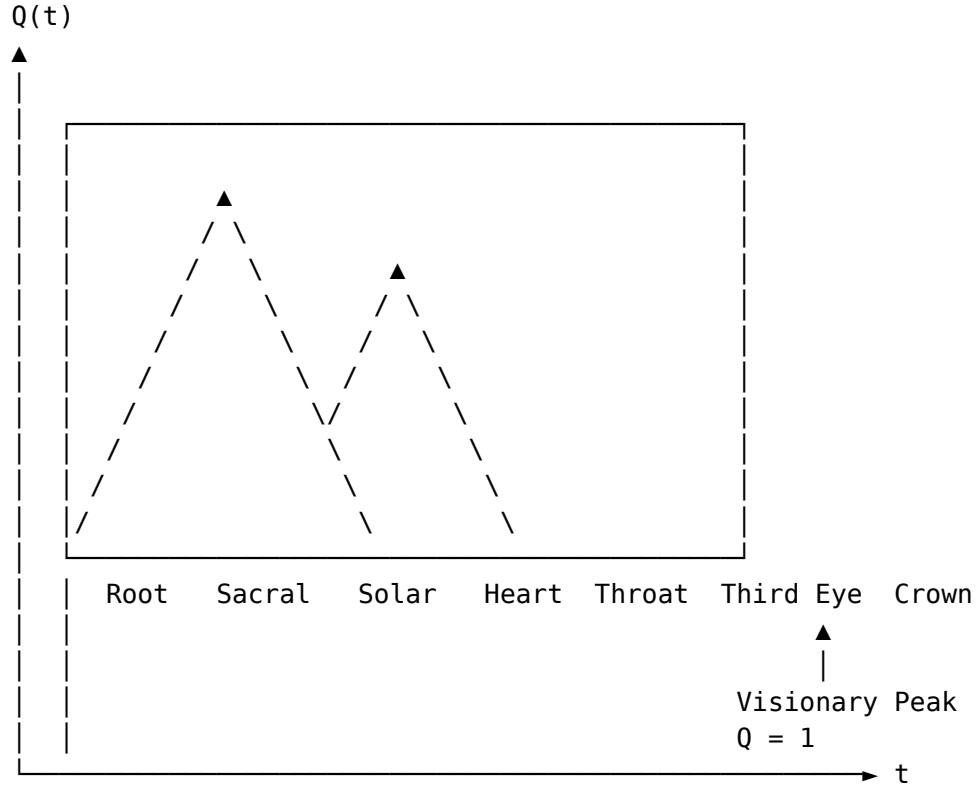
Figure 64: The qualia field during coherent \Phi -wave activation
