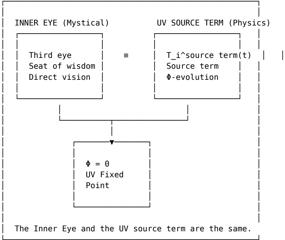
Figure 69: The identity Inner Eye = UV source term
