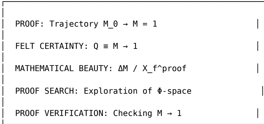
Figure 53: Proof theory from holographic dynamics
