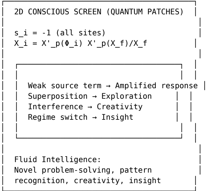
Figure 21: Fluid intelligence as the quantum regime
