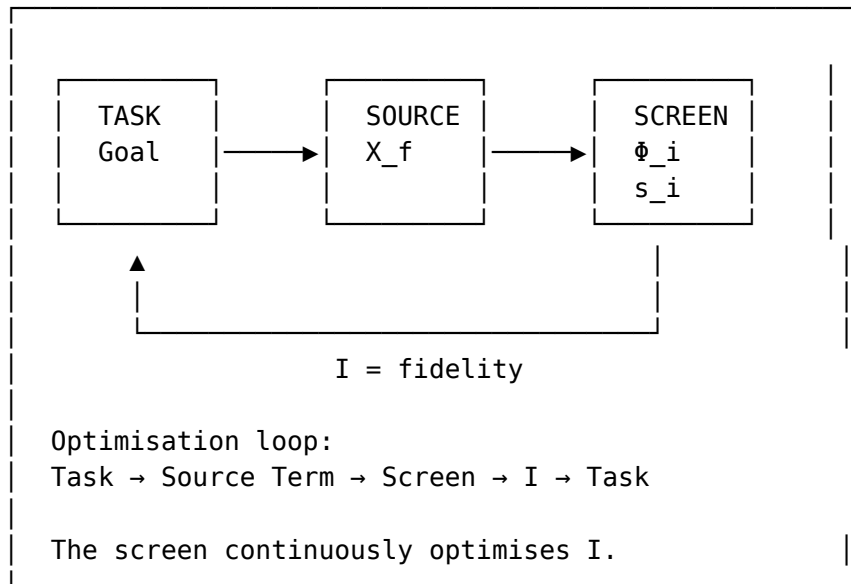
Figure 20: The intelligence optimisation cycle
