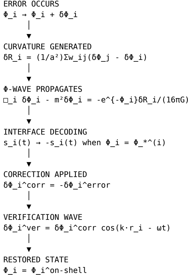
Figure 12: The complete error correction cycle
