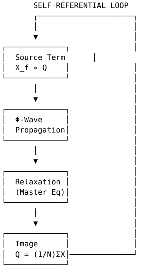
Figure 3: The self-referential loop of consciousness
