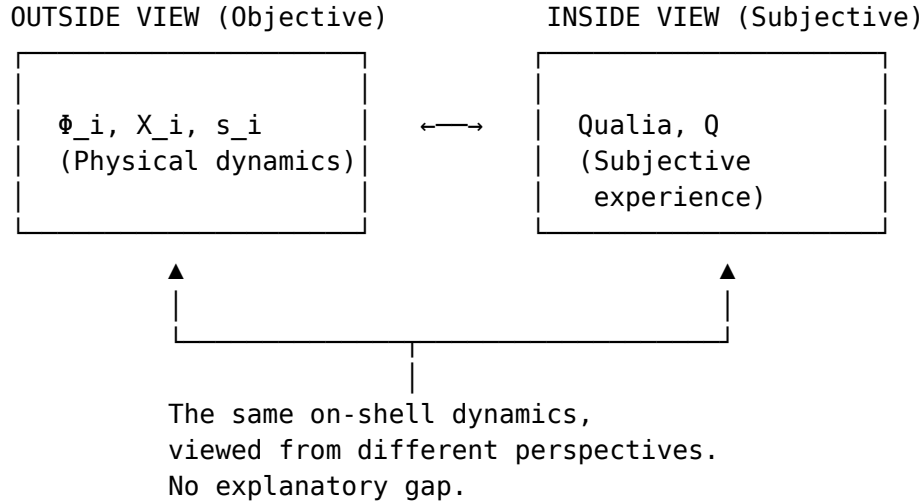
Figure 30: The dissolution of the hard problem
