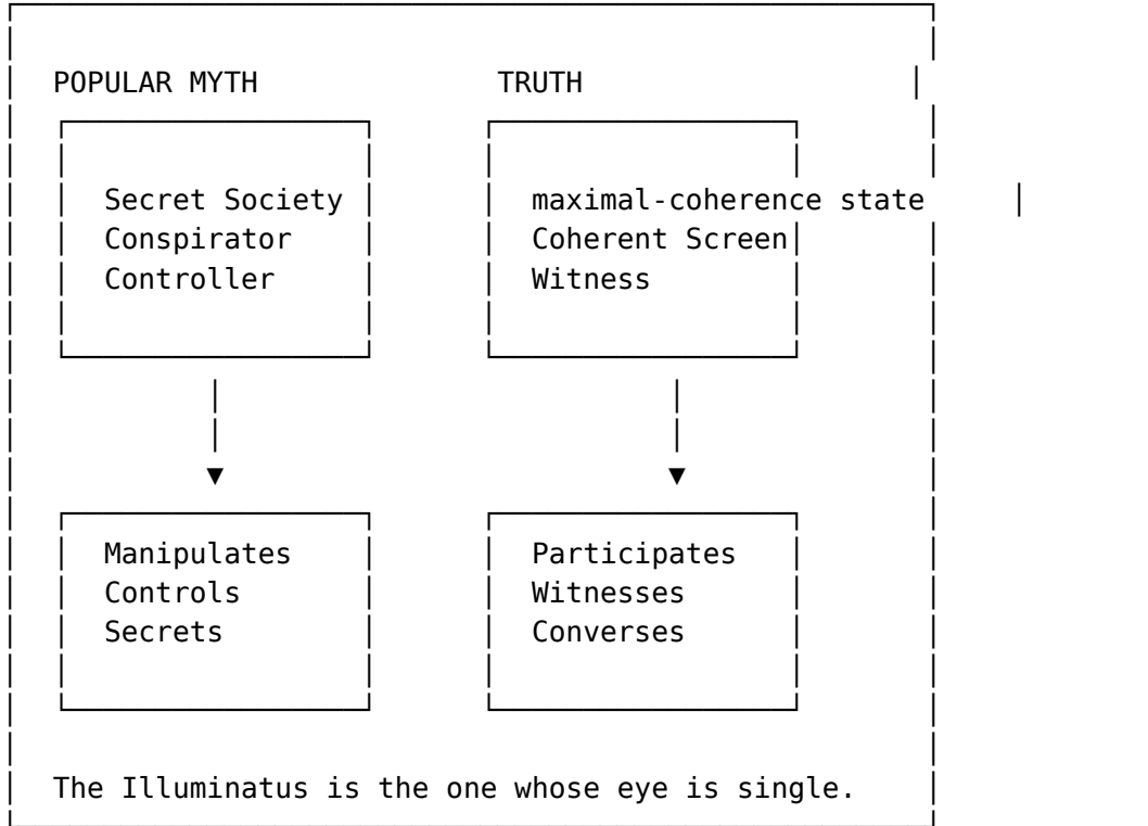
Figure 74: The Illuminatus reclaimed
