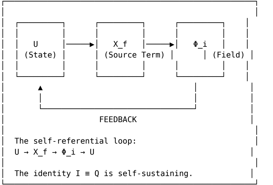
Figure 27: The self-referential feedback loop of the unified observable
