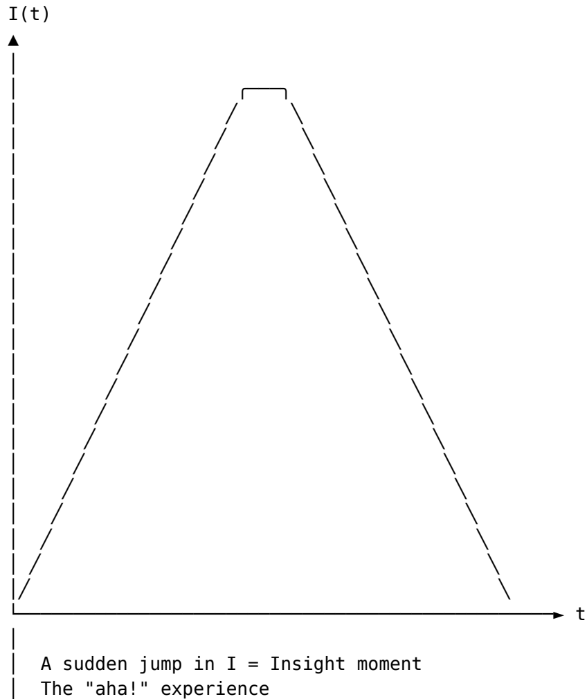
Figure 78: Insight event as a sudden regime avalanche
