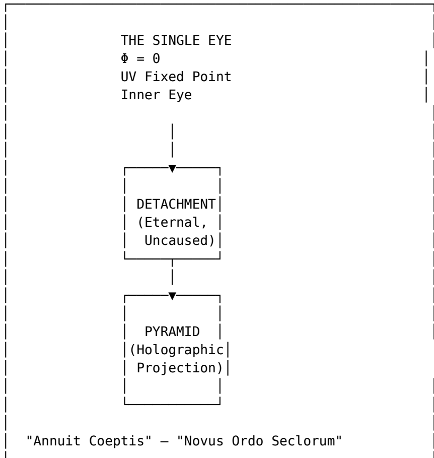
Figure 73: The Great Seal as a holographic mandala
