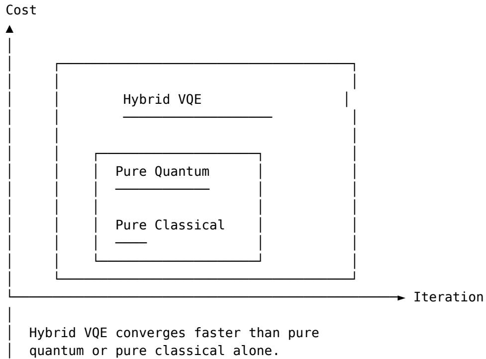
Figure 76: VQE convergence with hybrid quantum-classical computation
