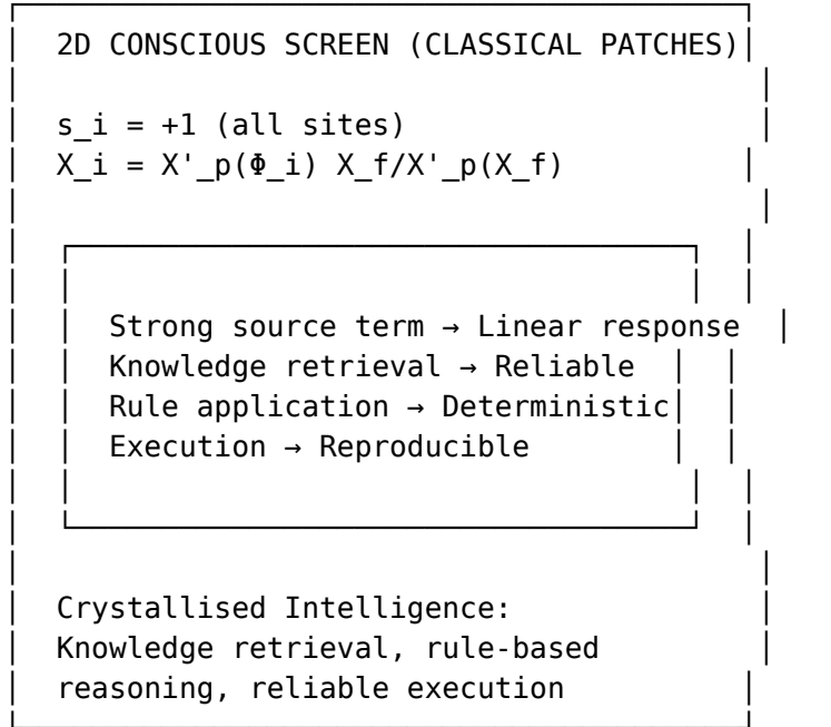
Figure 22: Crystallised intelligence as the classical regime
