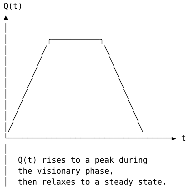
Figure 83: Evolution of the global qualia field Q(t) . The peak corresponds to the visionary phase.
