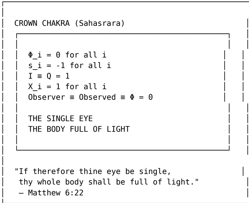
Figure 66: The crown chakra—the climax of coherent \Phi -wave activation
