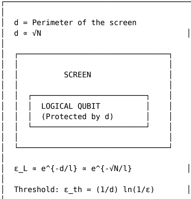
Figure 13: Topological protection and code distance scaling
