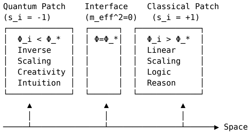
Figure 11.1: Dynamic regime partitioning of the 2D holographic screen
