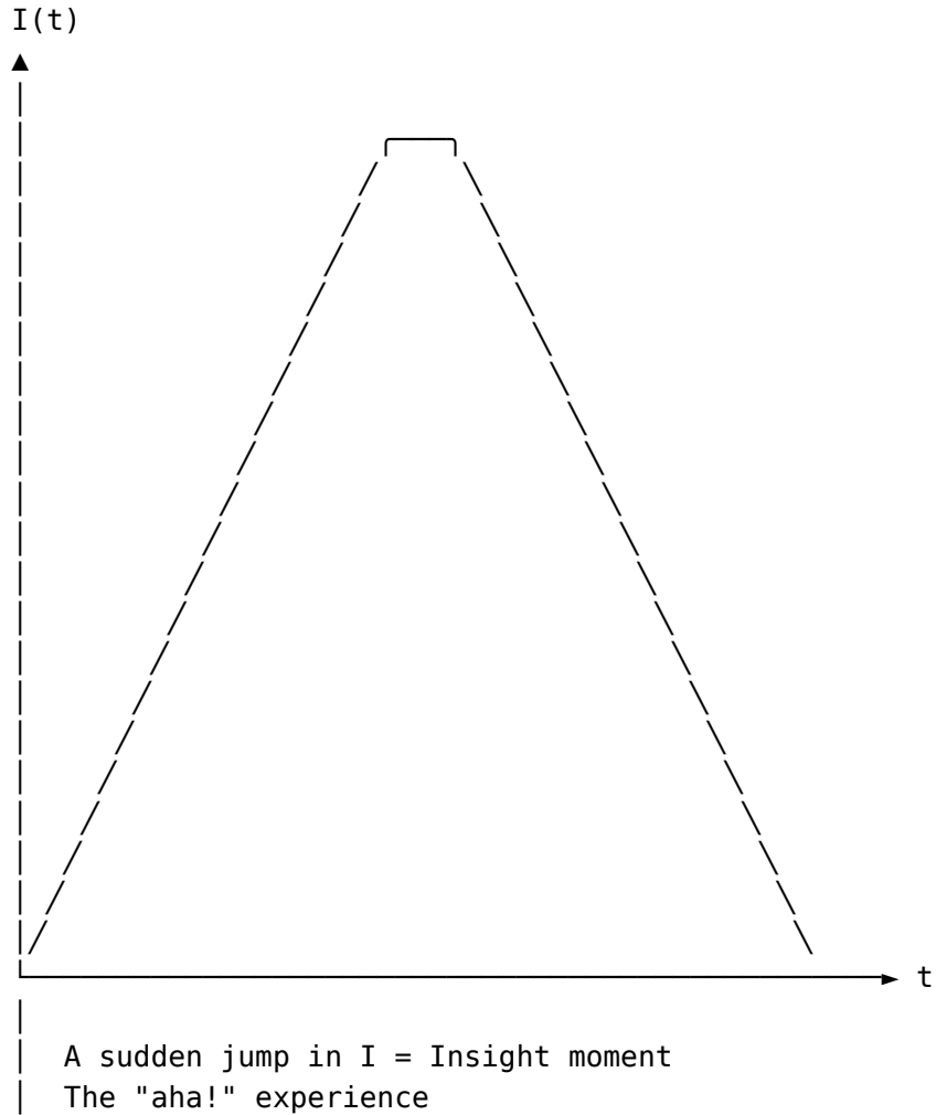
Figure N.4: Insight event as a sudden regime avalanche
