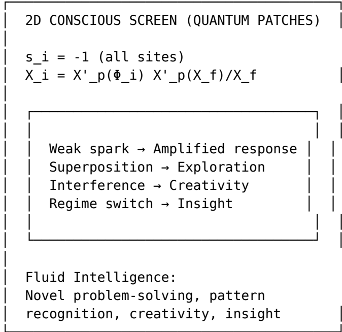
Figure 13.2: Fluid intelligence as the quantum regime
