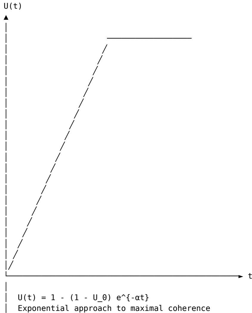
Figure 14.4: The transition to maximal coherence
