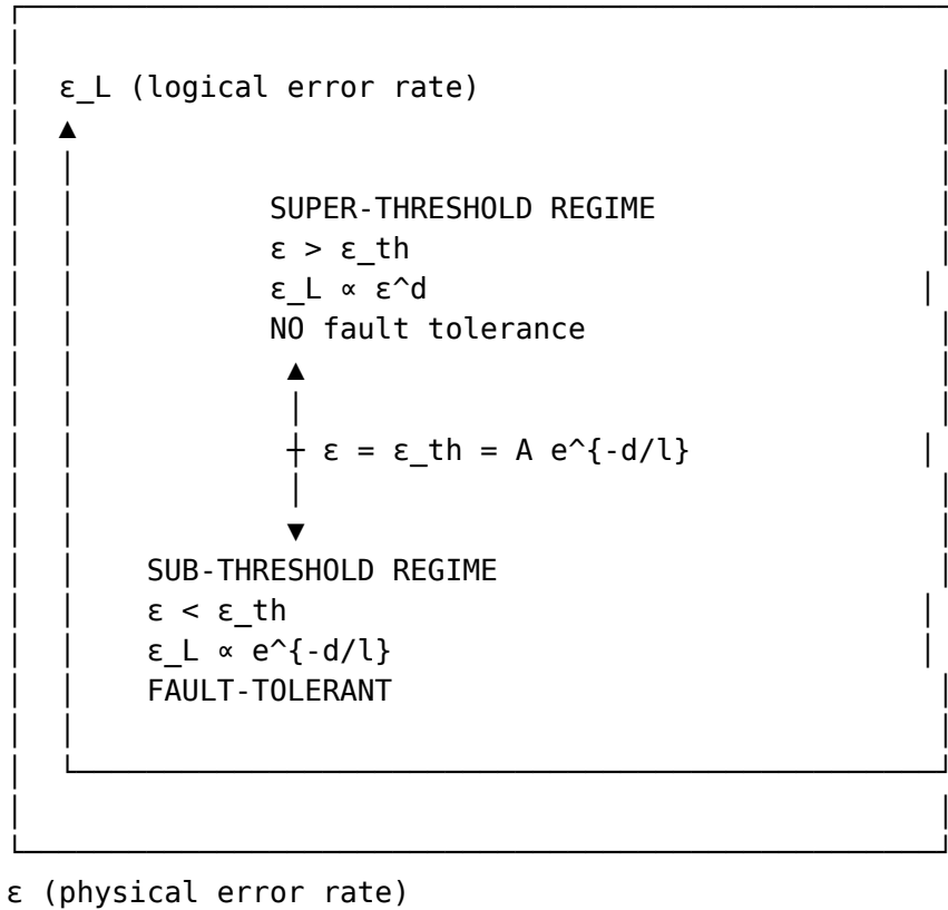
Figure 12.5: The fault-tolerance threshold and the two regimes
