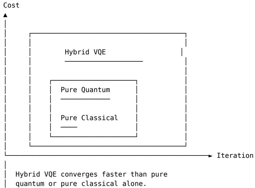
Figure N.2: VQE convergence with hybrid quantum-classical computation
