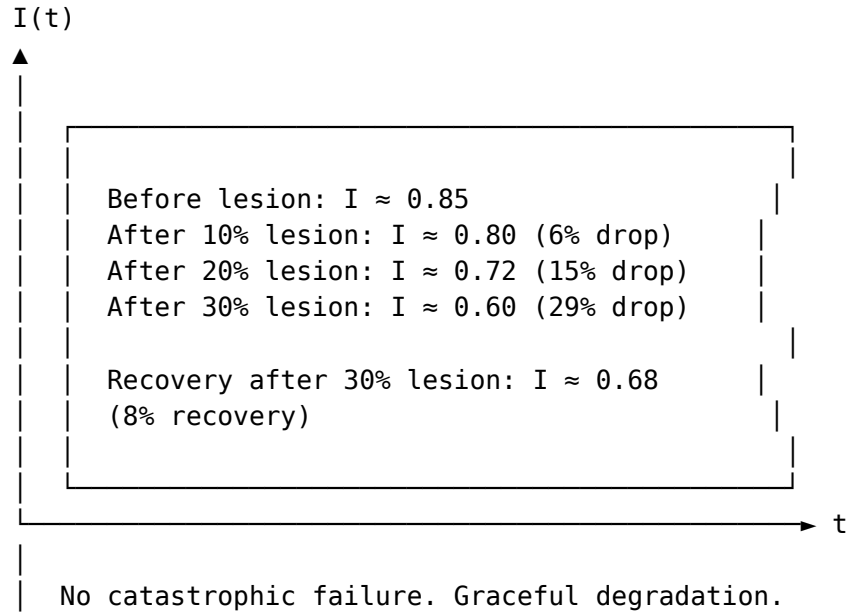
Figure N.5: Graceful degradation under focal lesions
