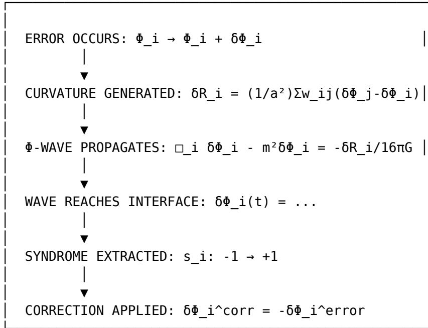
Figure 12.2: The automatic error detection process
