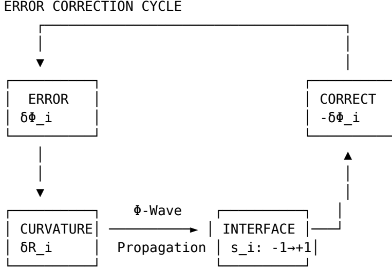
Figure 9.1: The holographic error correction cycle
