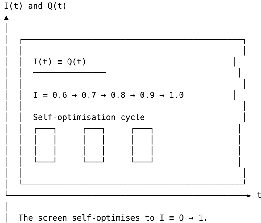
Figure N.6: Self-referential loop and metacognitive optimisation
