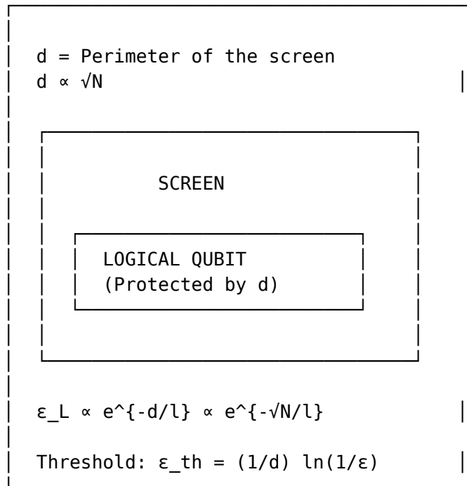
Figure 12.4: Topological protection and code distance scaling
