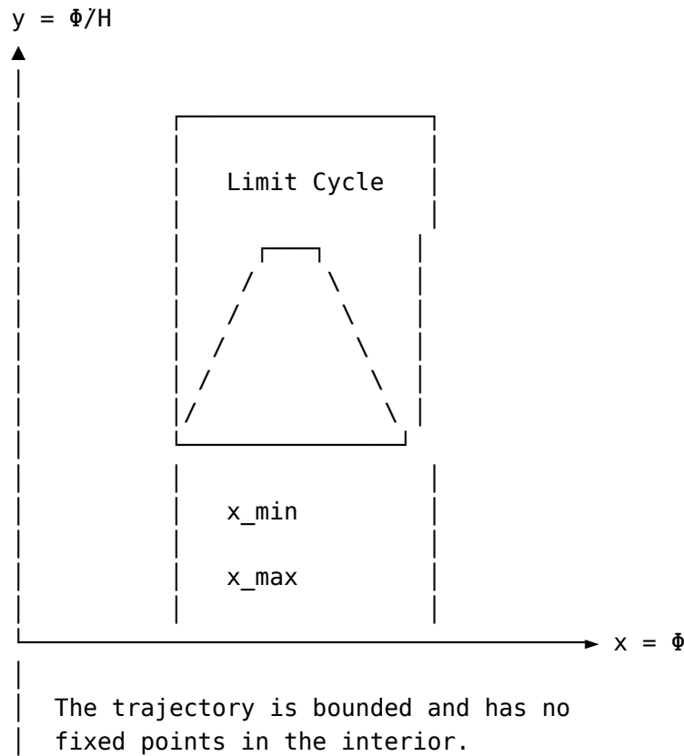
Figure 18.3: The reduced phase space with the limit cycle
