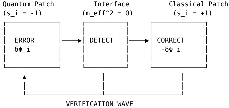
Figure 11.2: Error correction across the quantum-classical interface
