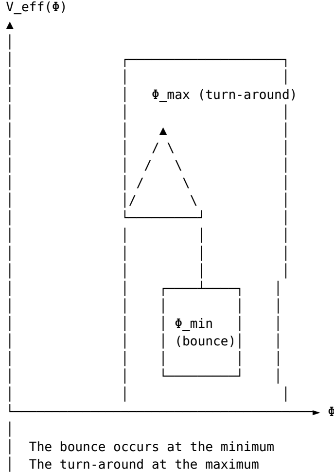
Figure 18.1: The effective potential and the bounce
