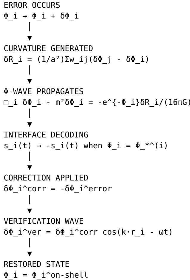
Figure 12.3: The complete error correction cycle
