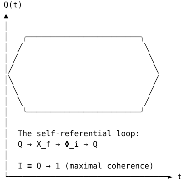
Figure S.4: The self-referential loop: Q \rightarrow X_f \rightarrow \Phi_i \rightarrow Q . The system reaches maximal coherence I \equiv Q \rightarrow 1 .
