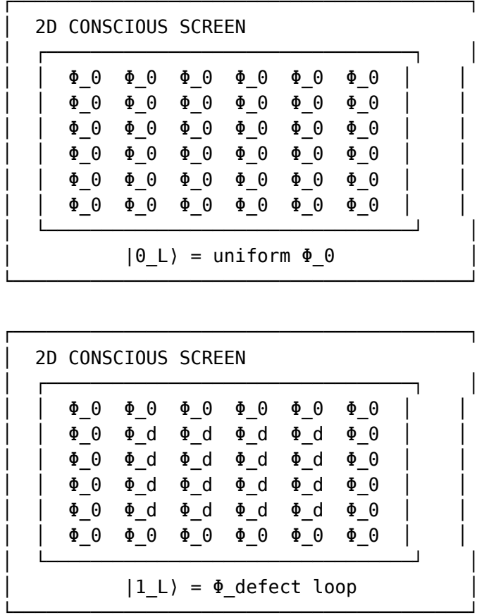
Figure 12.1: Logical qubit encoding in global \Phi -patterns
