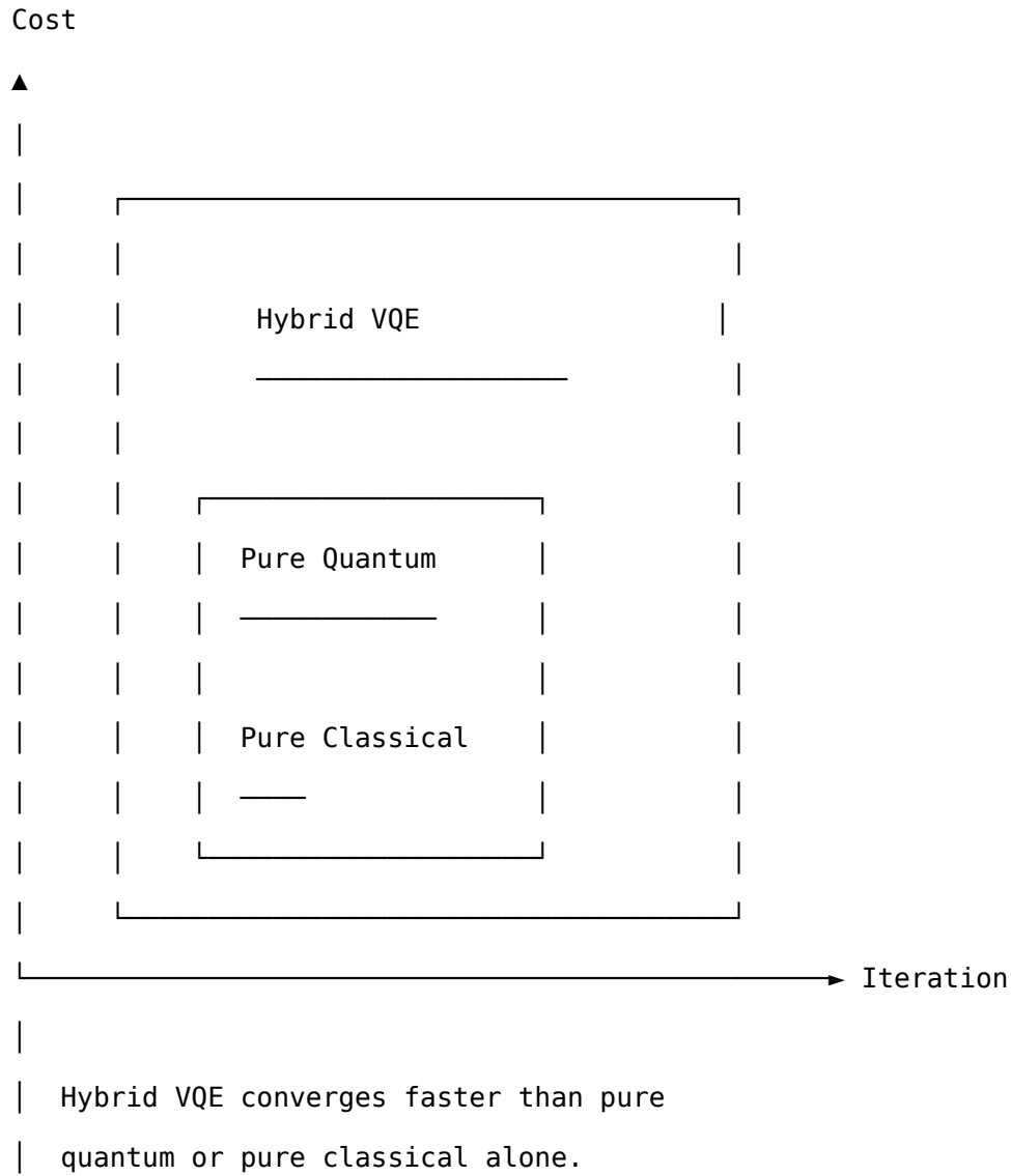
FIG. 76. VQE convergence with hybrid quantum-classical computation
