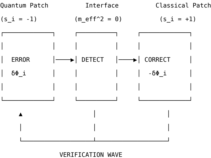
FIG. 7. Error correction across the quantum-classical interface
