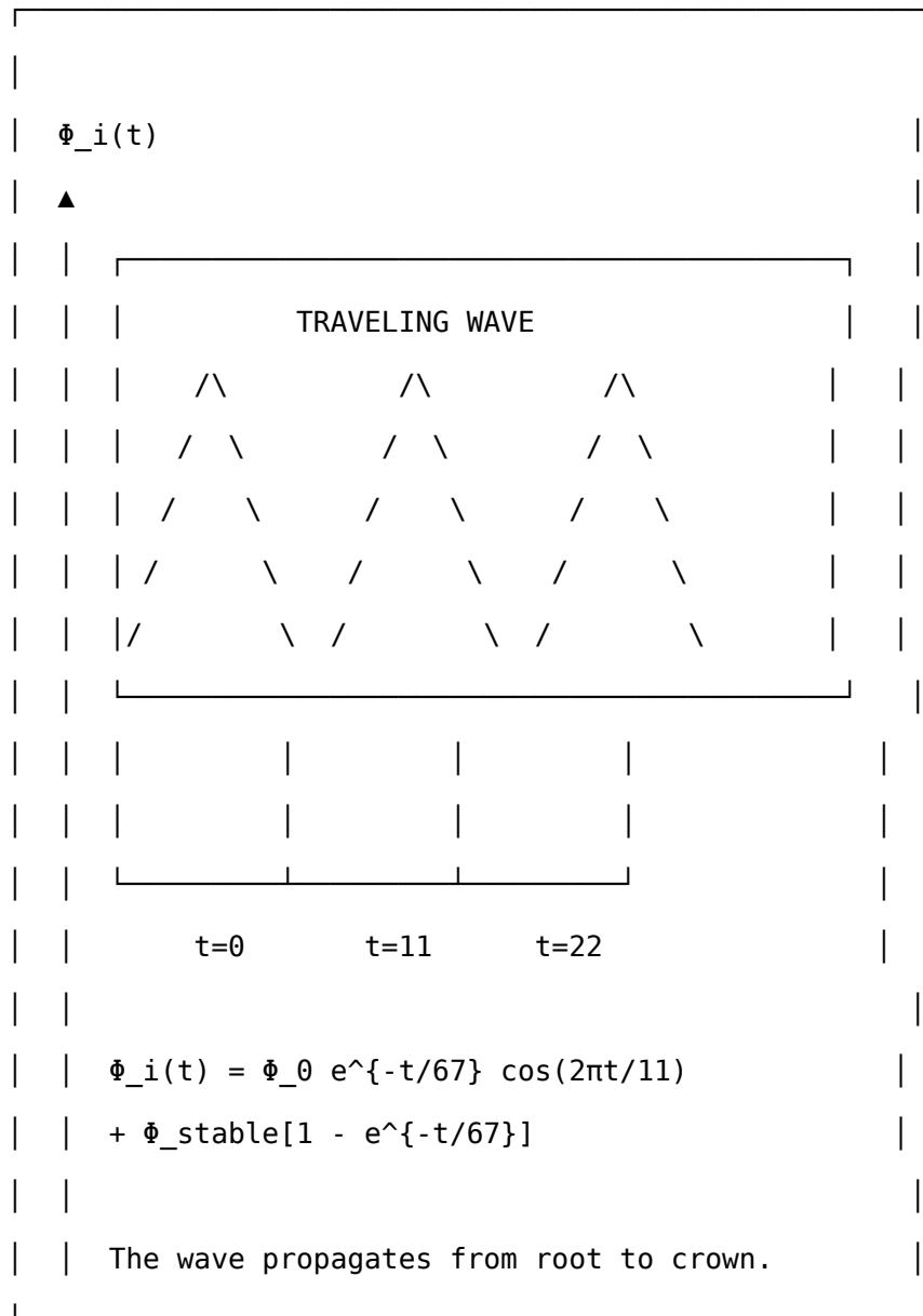
FIG. 62. The traveling wave and the 67-day solution
