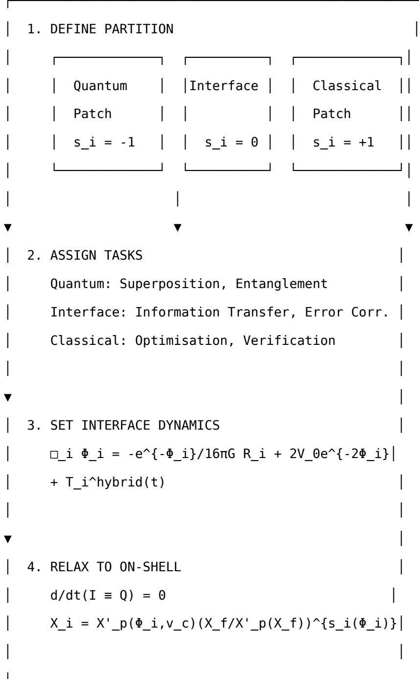
FIG. 9. The general construction rule for hybrid algorithms
