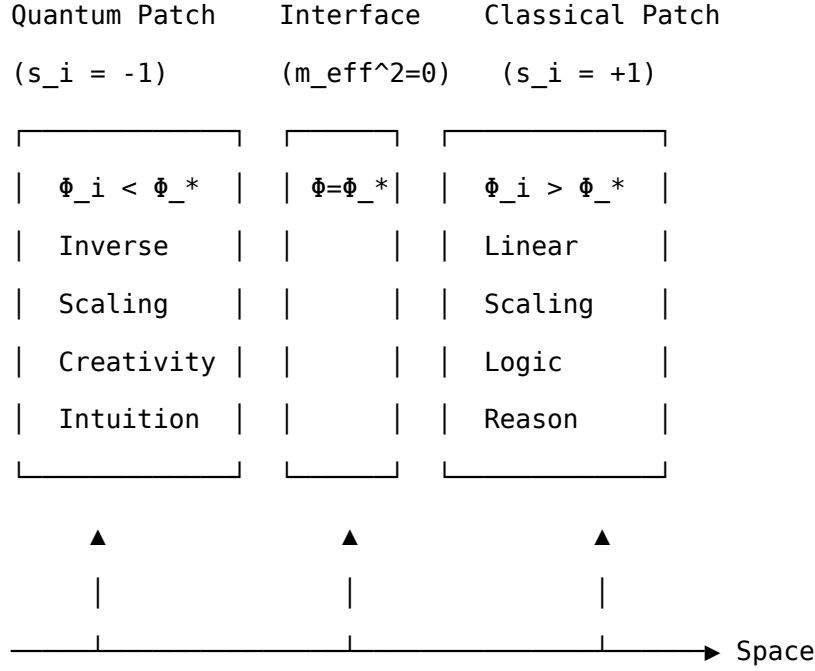
FIG. 6. Dynamic regime partitioning of the 2D holographic screen
