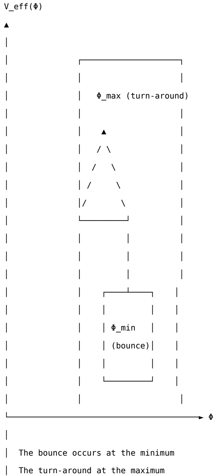
FIG. 56. The effective potential and the bounce
