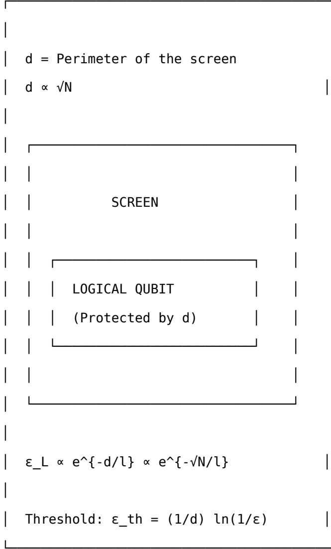
FIG. 13. Topological protection and code distance scaling
