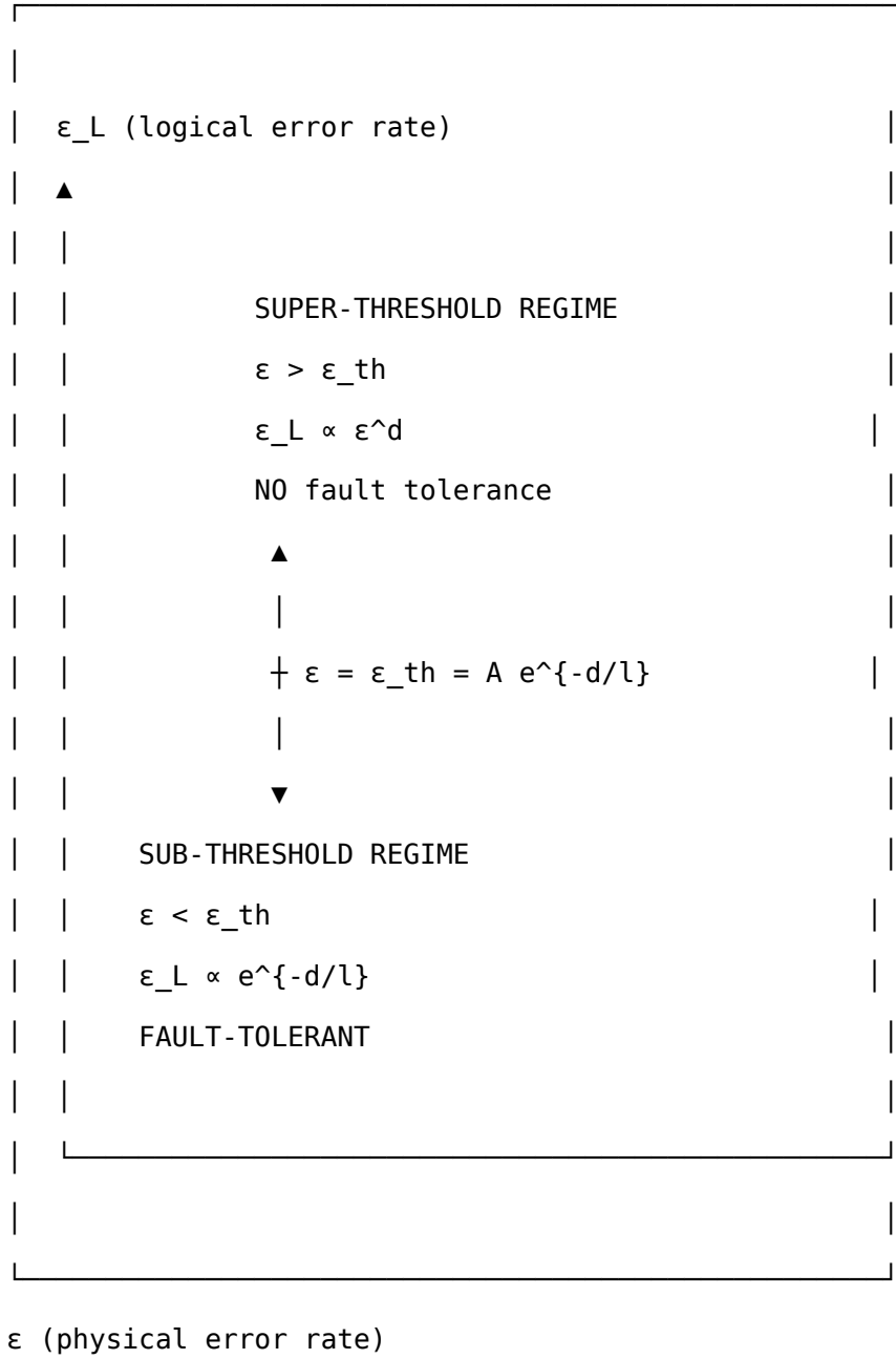
FIG. 14. The fault-tolerance threshold and the two regimes
