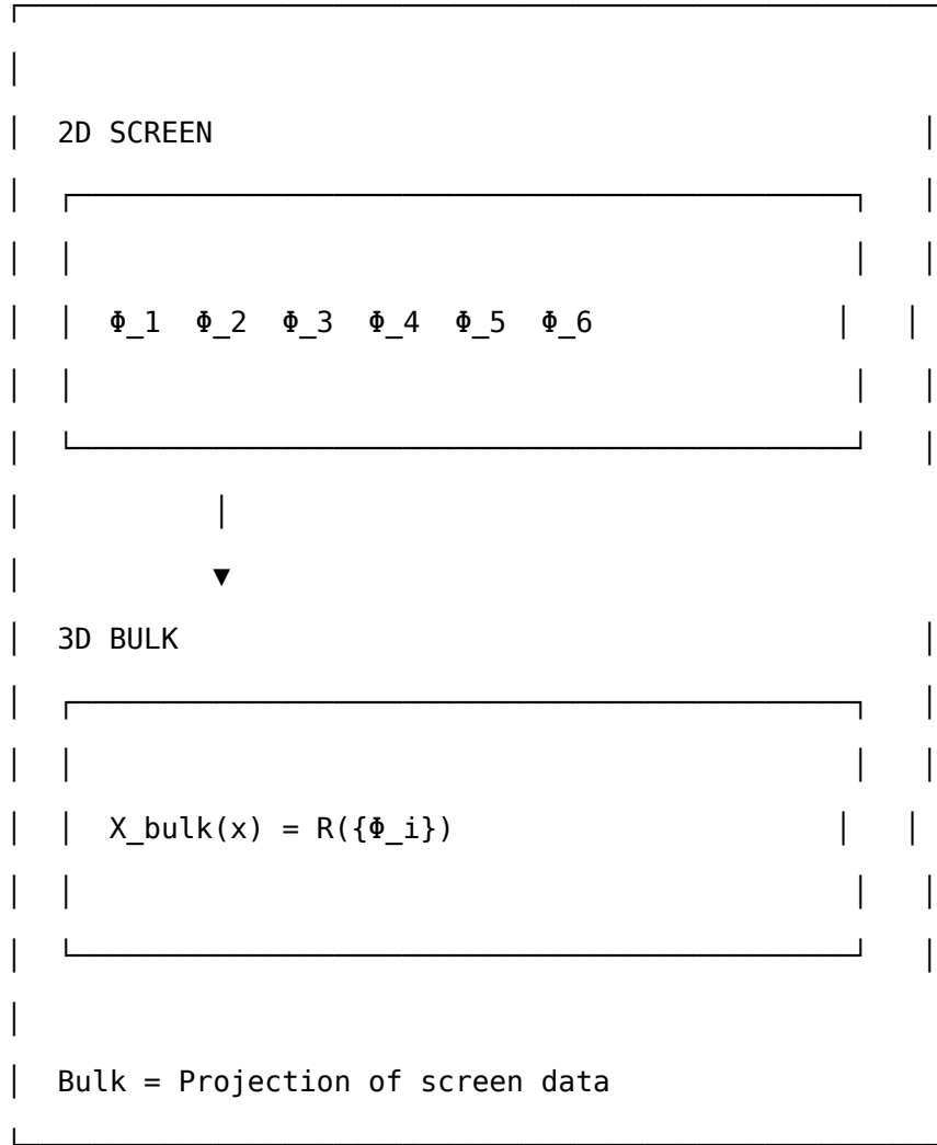
FIG. 34. Holographic projection from the 2D screen to the bulk
