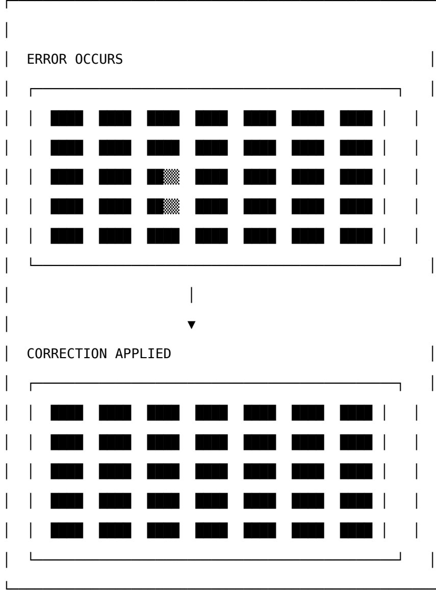
FIG. 77. Error correction on the holographic lattice
