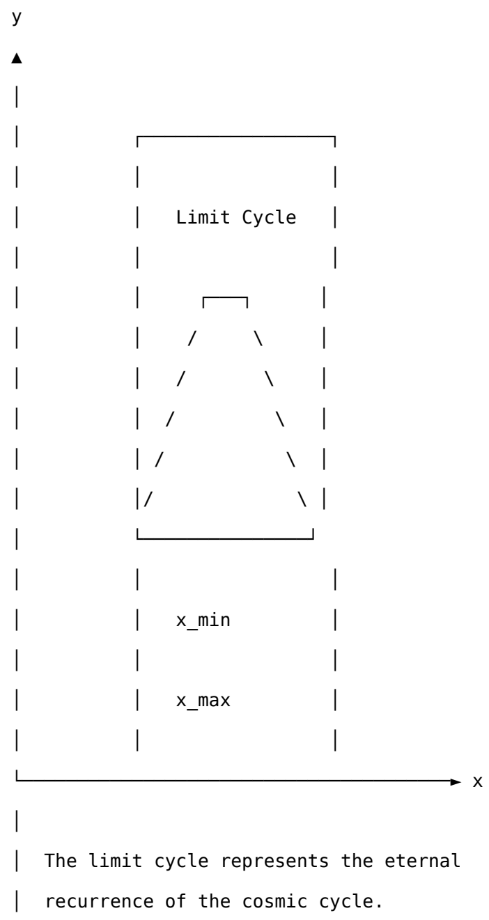
FIG. 59. The limit cycle in the reduced phase space
