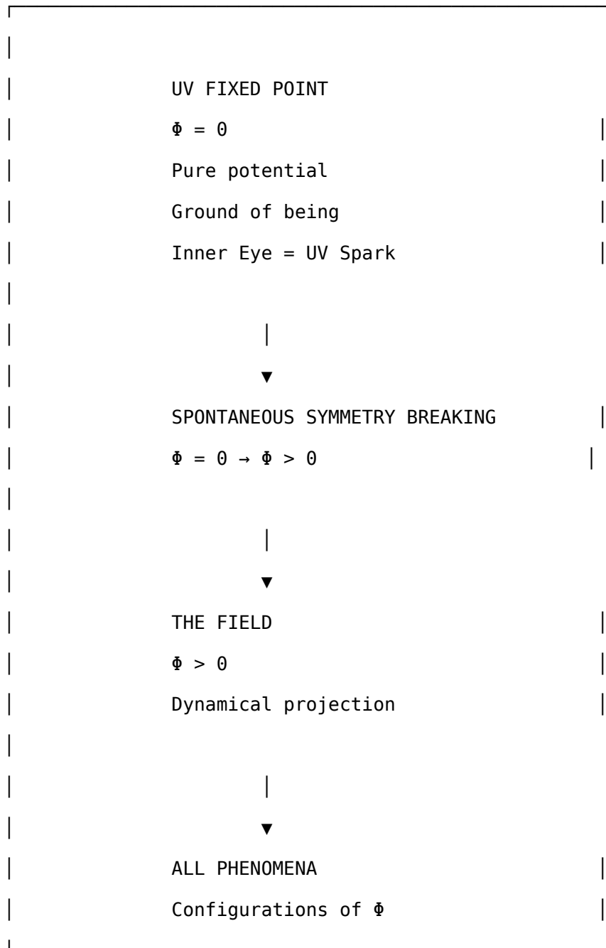
FIG. 35. The UV fixed point as the source of all phenomena
