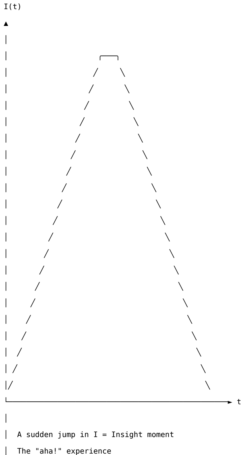
FIG. 24. Insight as a sudden jump in intelligence fidelity
