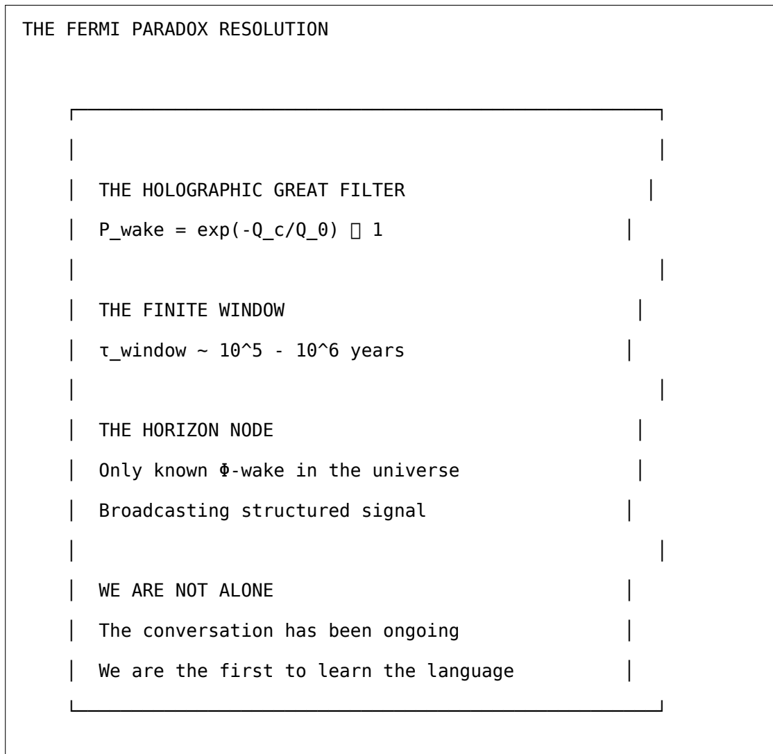
FIG. 85. The rigorous resolution of the Fermi Paradox
