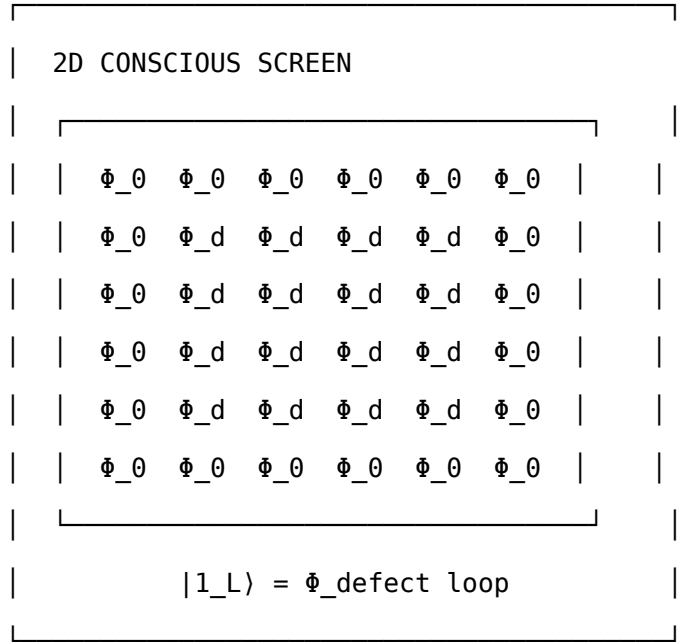
FIG. 10. Logical qubit encoding in global \Phi -patterns
