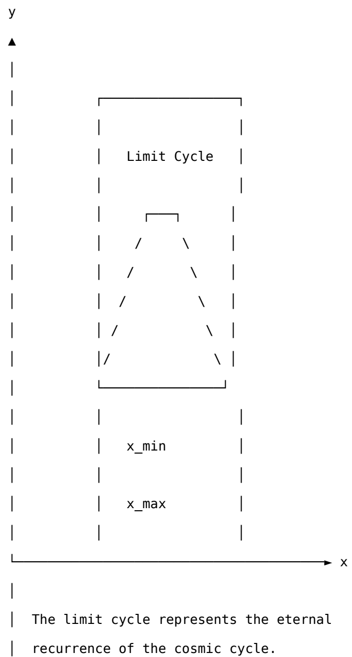
FIG. 59. The limit cycle in the reduced phase space
