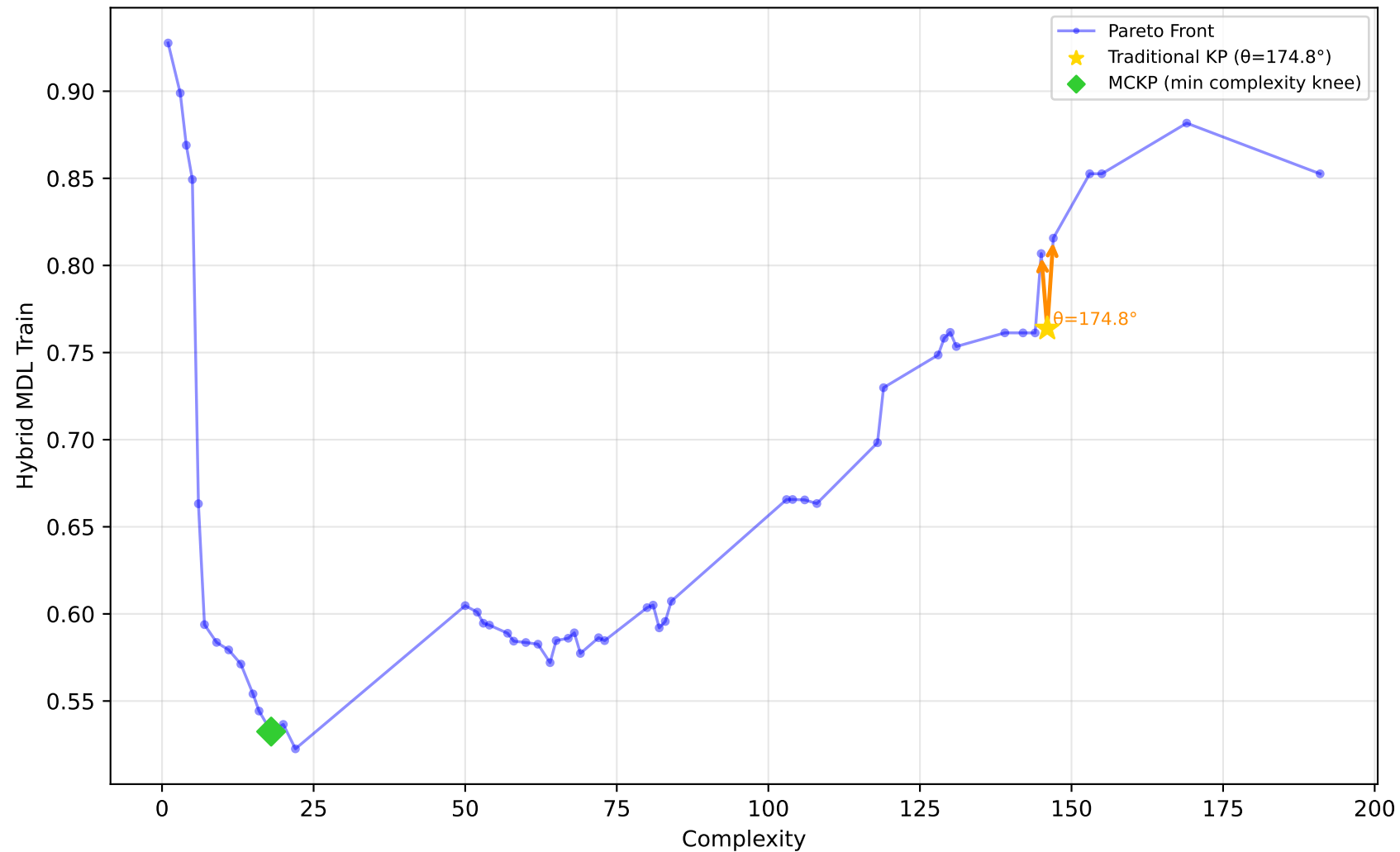
589_fri_c2_1000_25 - Run 10 - MVP - Hybrid MDL Train \lambda_1=0.30, \lambda_2=0.00, \lambda_3=0.20 | Difficulty: 1.00 | Method: hmr
