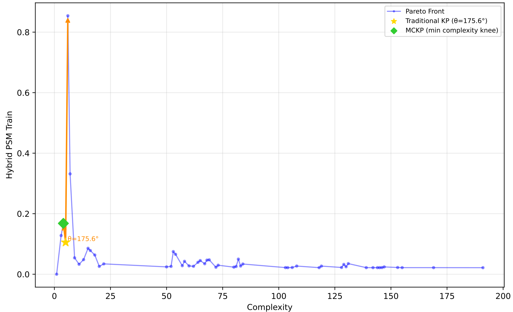
589_fri_c2_1000_25 - Run 10 - MVP - Hybrid PSM Train \lambda_1=0.30, \lambda_2=0.00, \lambda_3=0.20 | Difficulty: 1.00 | Method: hmr
