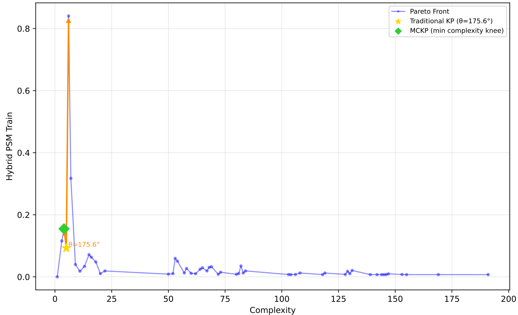
589_fri_c2_1000_25 - Run 10 - SVP - Hybrid PSM Train \lambda_1=0.10, \bar{\lambda}_2=0.00, \bar{\lambda}_3=0.10 | Difficulty: 1.00 | Method: hmr
