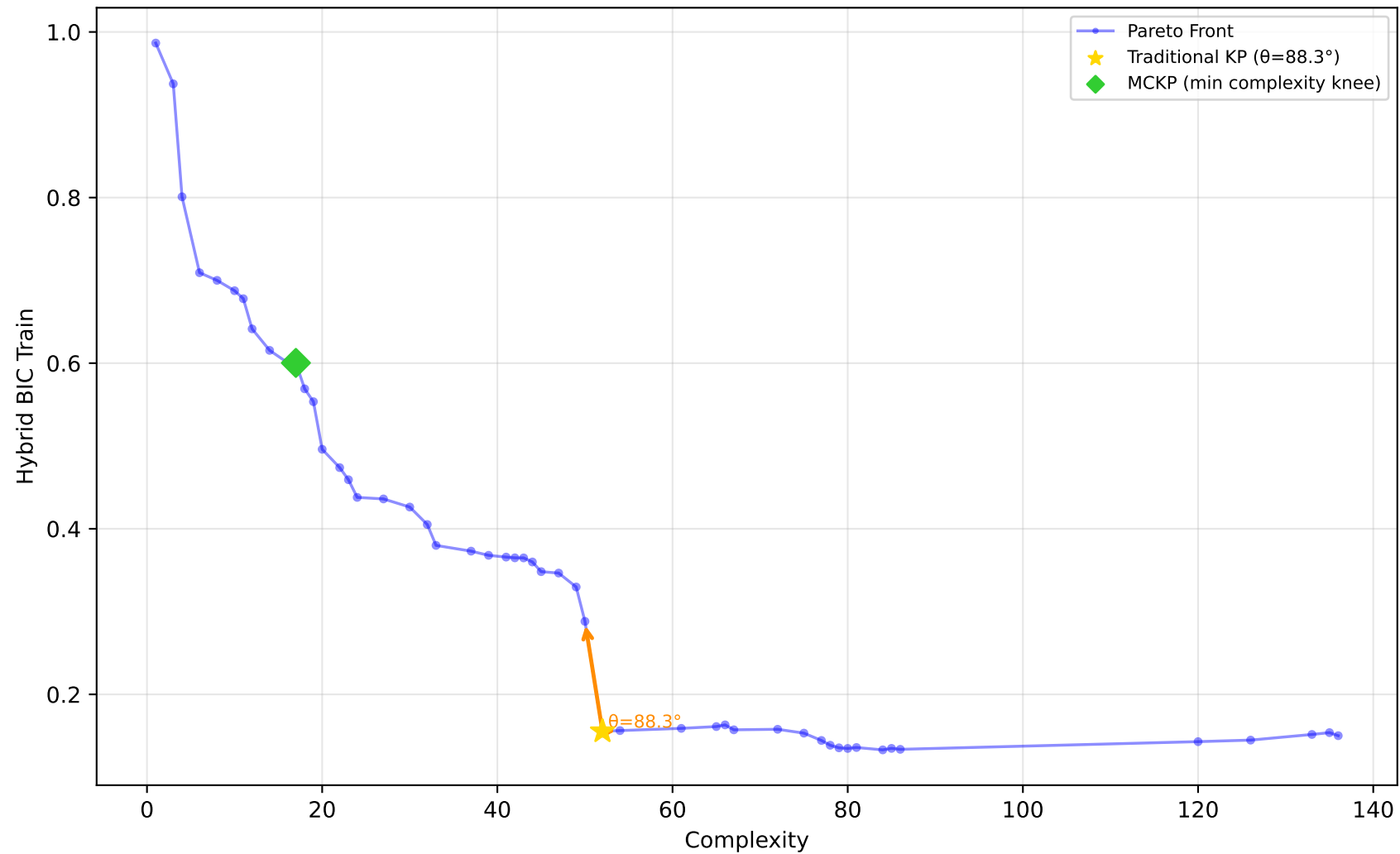
589_fri_c2_1000_25 - Run 11 - MVP - Hybrid BIC Train \lambda_1=0.00, \bar{\lambda}_2=0.00, \bar{\lambda}_3=0.00 | Difficulty: 1.00 | Method: hmr
