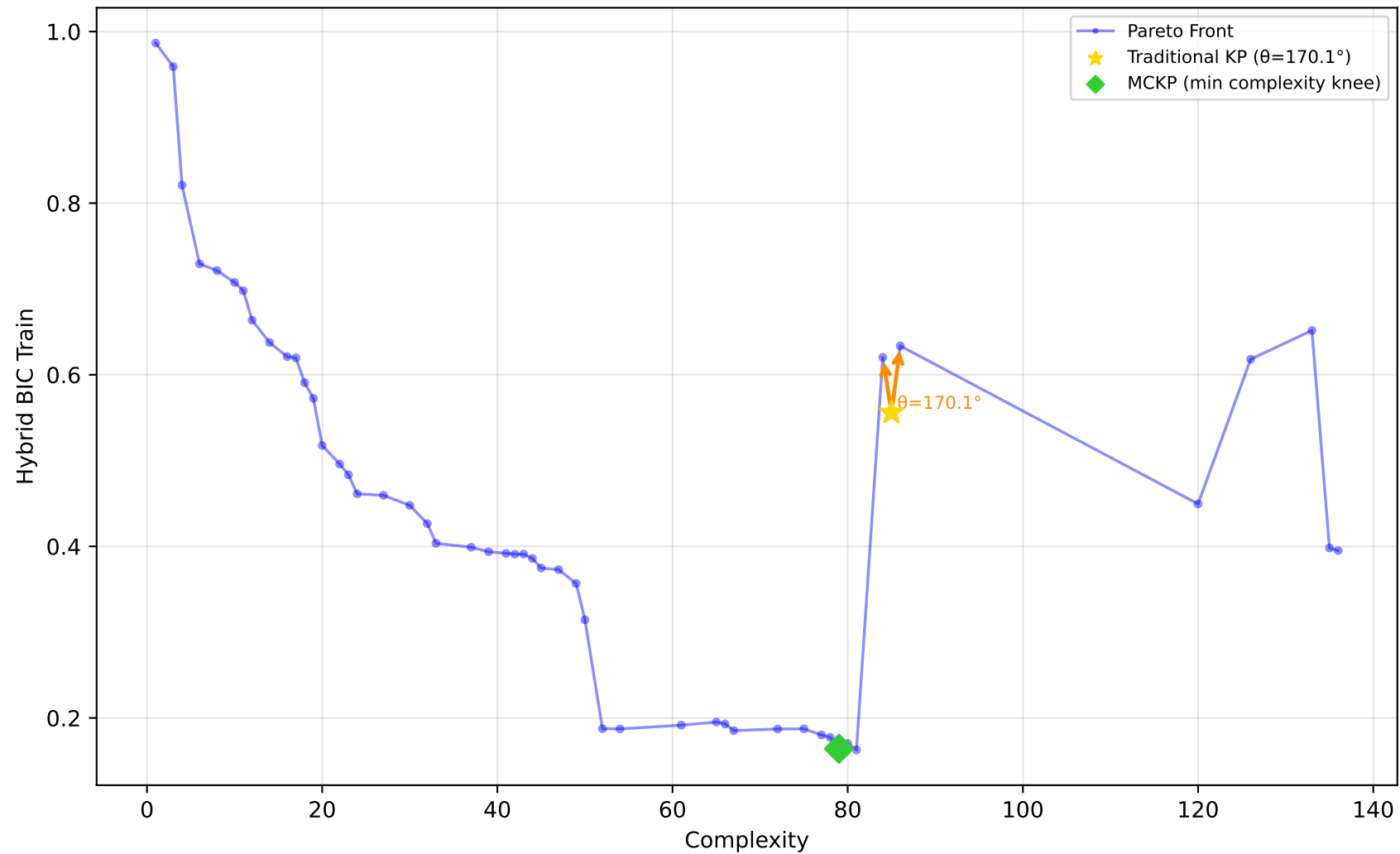
589_fri_c2_1000_25 - Run 11 - MVP - Hybrid BIC Train \lambda_1=0.30, \bar{\lambda}_2=0.00, \bar{\lambda}_3=0.20 | Difficulty: 1.00 | Method: hmr
