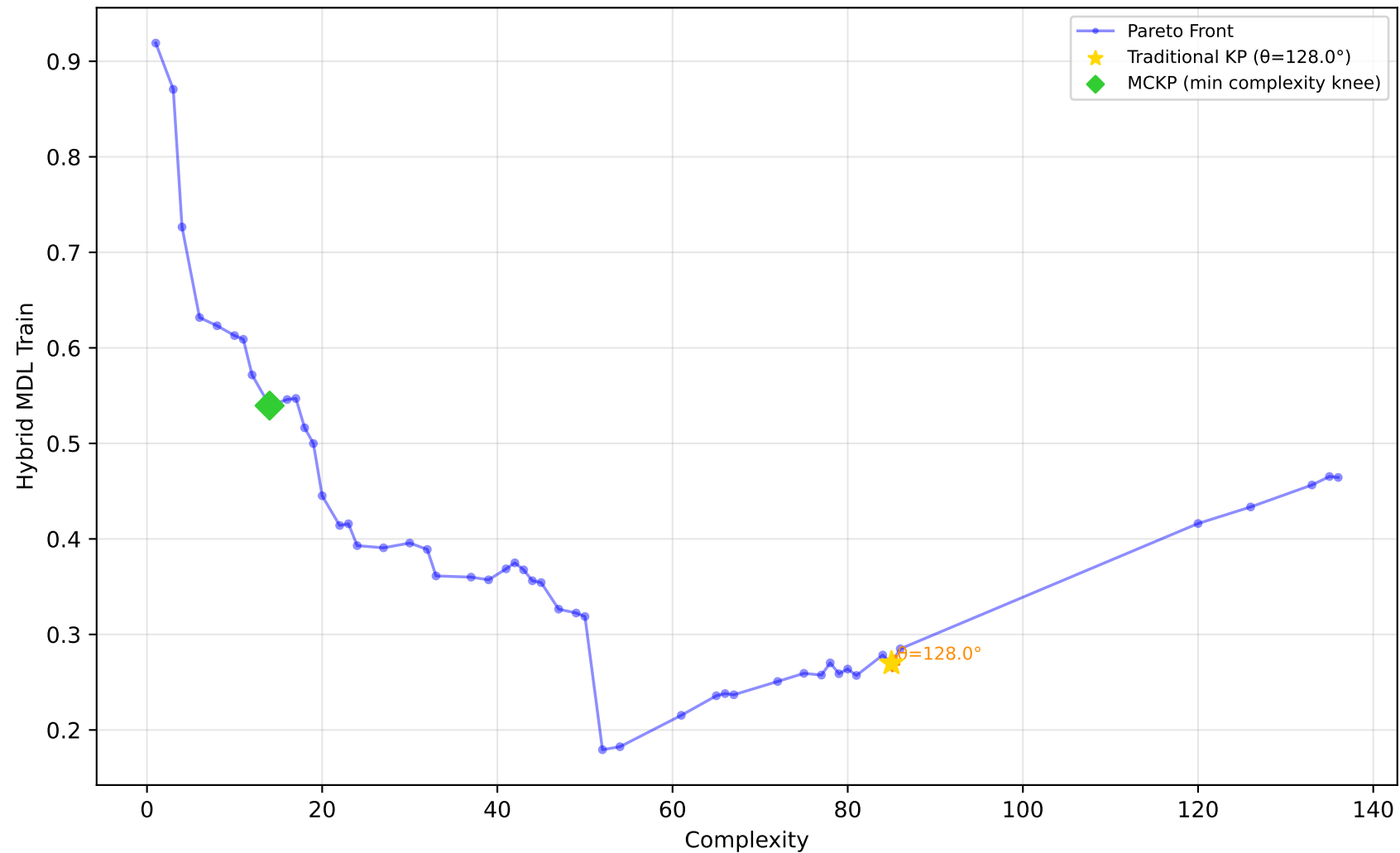
589_fri_c2_1000_25 - Run 11 - MVP - Hybrid MDL Train \lambda_1=0.00, \lambda_2=0.00, \lambda_3=0.00 | Difficulty: 1.00 | Method: hmr
