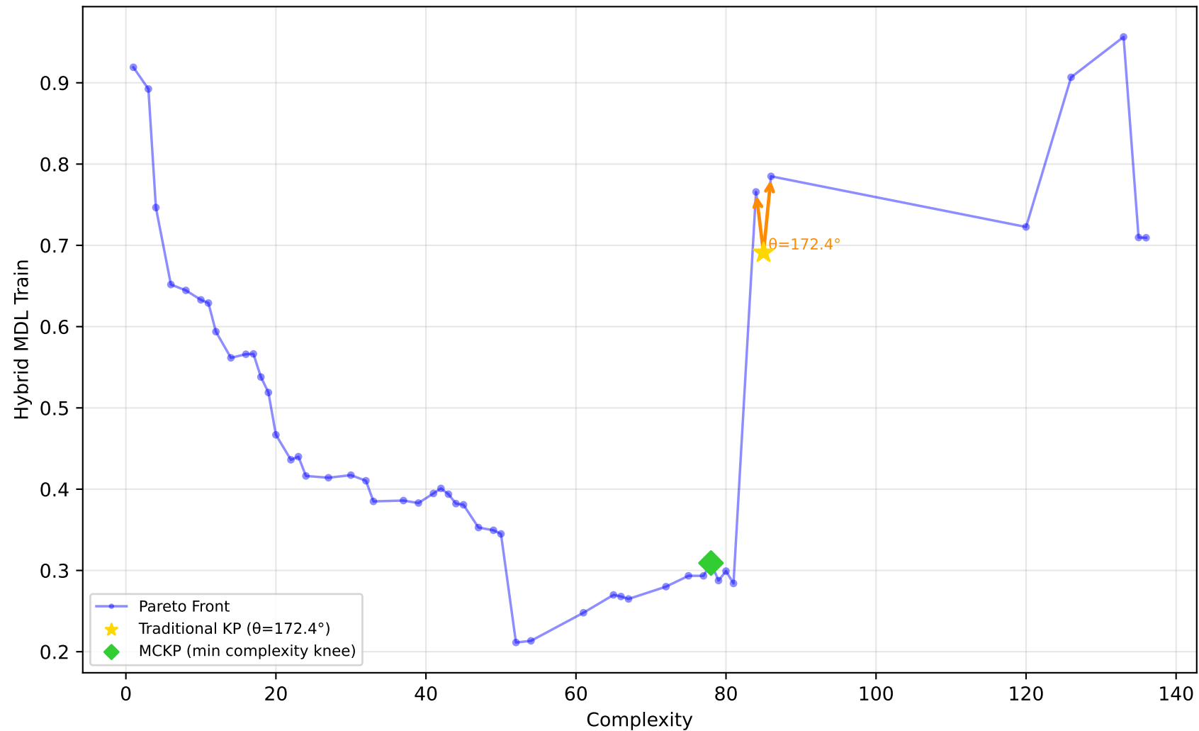
589_fri_c2_1000_25 - Run 11 - MVP - Hybrid MDL Train \lambda_1=0.30, \lambda_2=0.00, \lambda_3=0.20 | Difficulty: 1.00 | Method: hmr
