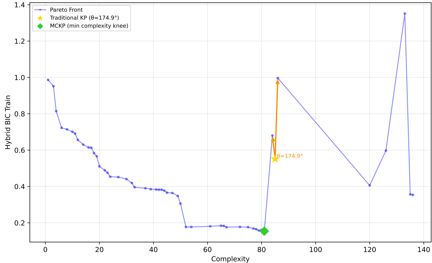
589_fri_c2_1000_25 - Run 11 - SVP - Hybrid BIC Train \lambda_1=0.20, \bar{\lambda}_2=0.00, \bar{\lambda}_3=1.00 | Difficulty: 1.00 | Method: hmr
