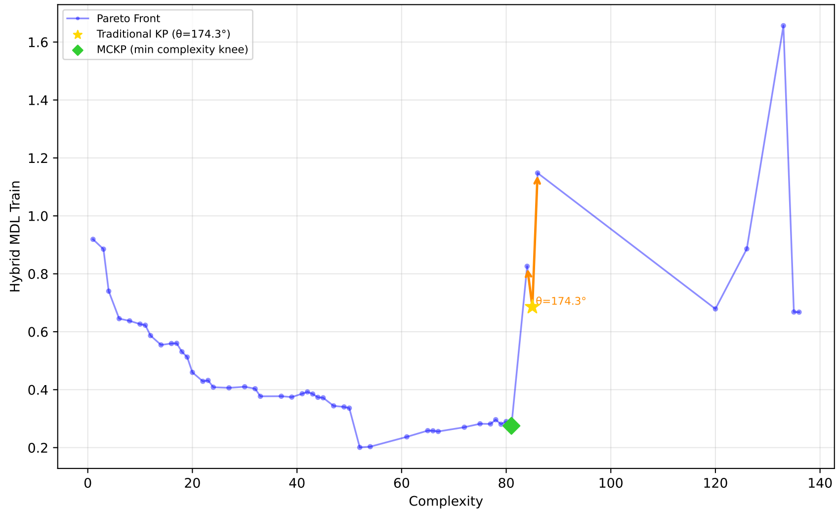
589_fri_c2_1000_25 - Run 11 - SVP - Hybrid MDL Train \lambda_1=0.20, \lambda_2=0.00, \lambda_3=1.00 | Difficulty: 1.00 | Method: hmr
