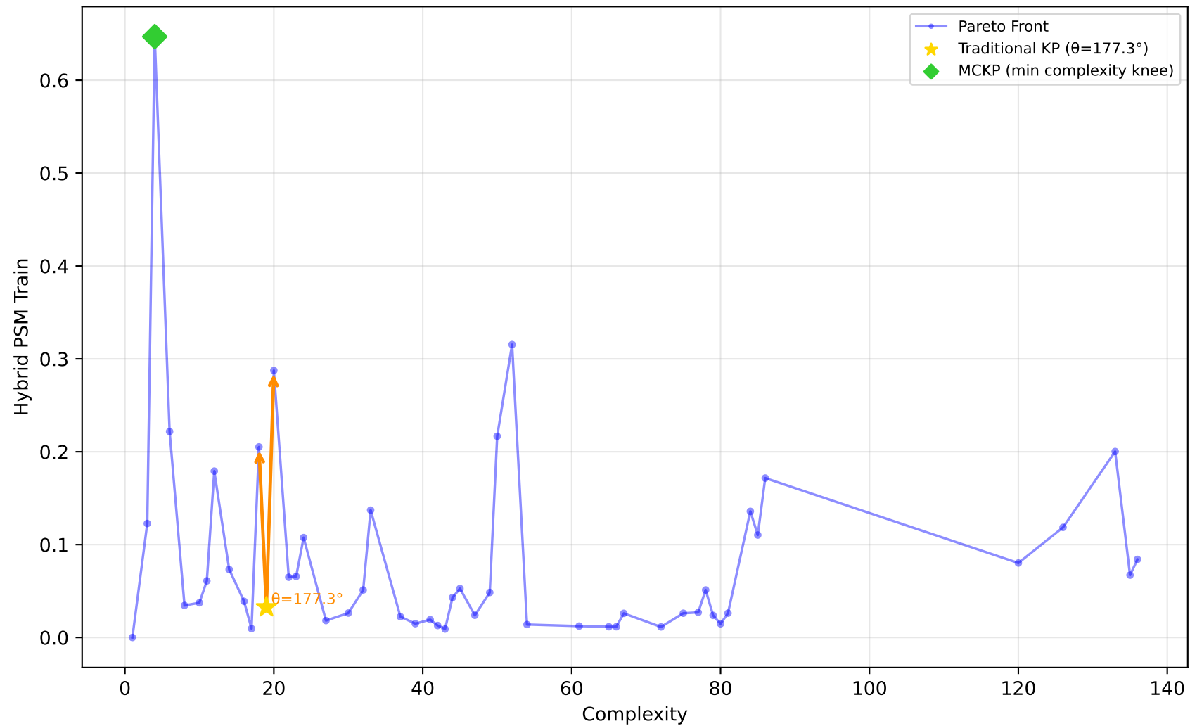
589_fri_c2_1000_25 - Run 11 - SVP - Hybrid PSM Train \lambda_1=0.10, \bar{\lambda}_2=0.00, \bar{\lambda}_3=0.10 | Difficulty: 1.00 | Method: hmr
