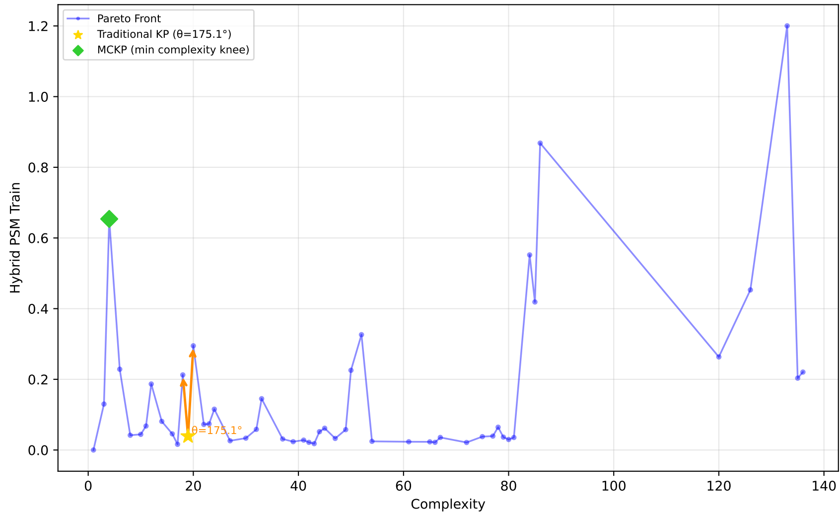
589_fri_c2_1000_25 - Run 11 - SVP - Hybrid PSM Train \lambda_1=0.20, \bar{\lambda}_2=0.00, \bar{\lambda}_3=1.00 | Difficulty: 1.00 | Method: hmr
