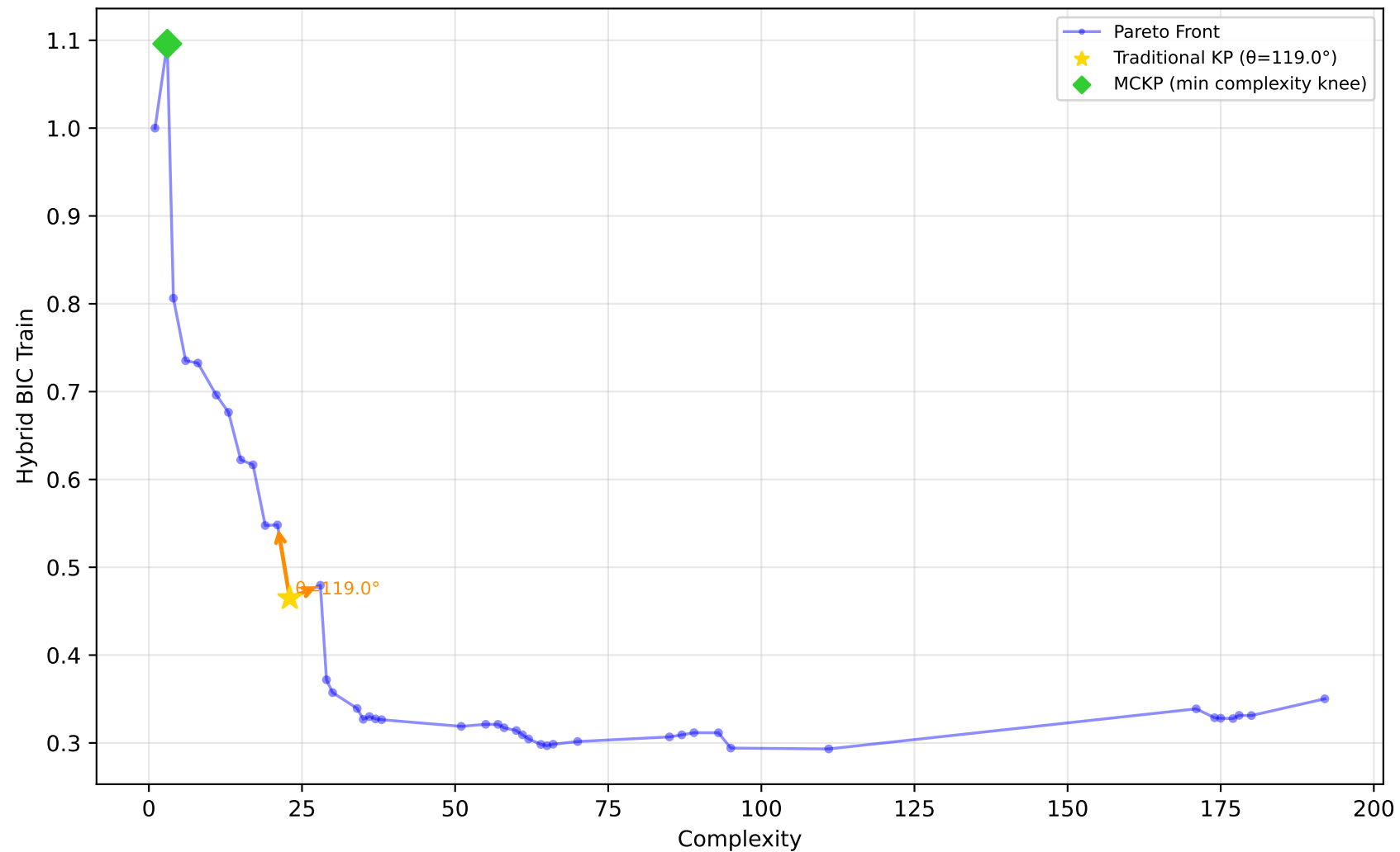
589_fri_c2_1000_25 - Run 12 - MVP - Hybrid BIC Train \lambda_1=0.30, \bar{\lambda}_2=0.00, \bar{\lambda}_3=0.20 | Difficulty: 1.00 | Method: hmr
