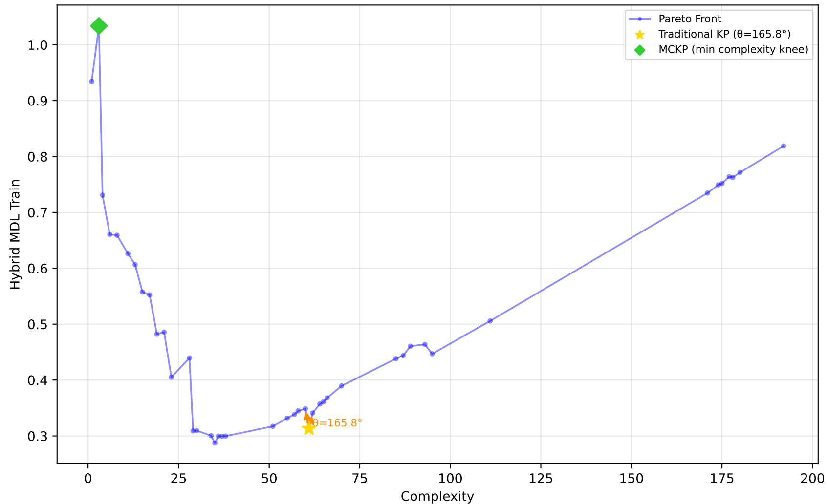
589_fri_c2_1000_25 - Run 12 - MVP - Hybrid MDL Train \lambda_1=0.30, \bar{\lambda}_2=0.00, \bar{\lambda}_3=0.20 | Difficulty: 1.00 | Method: hmr
