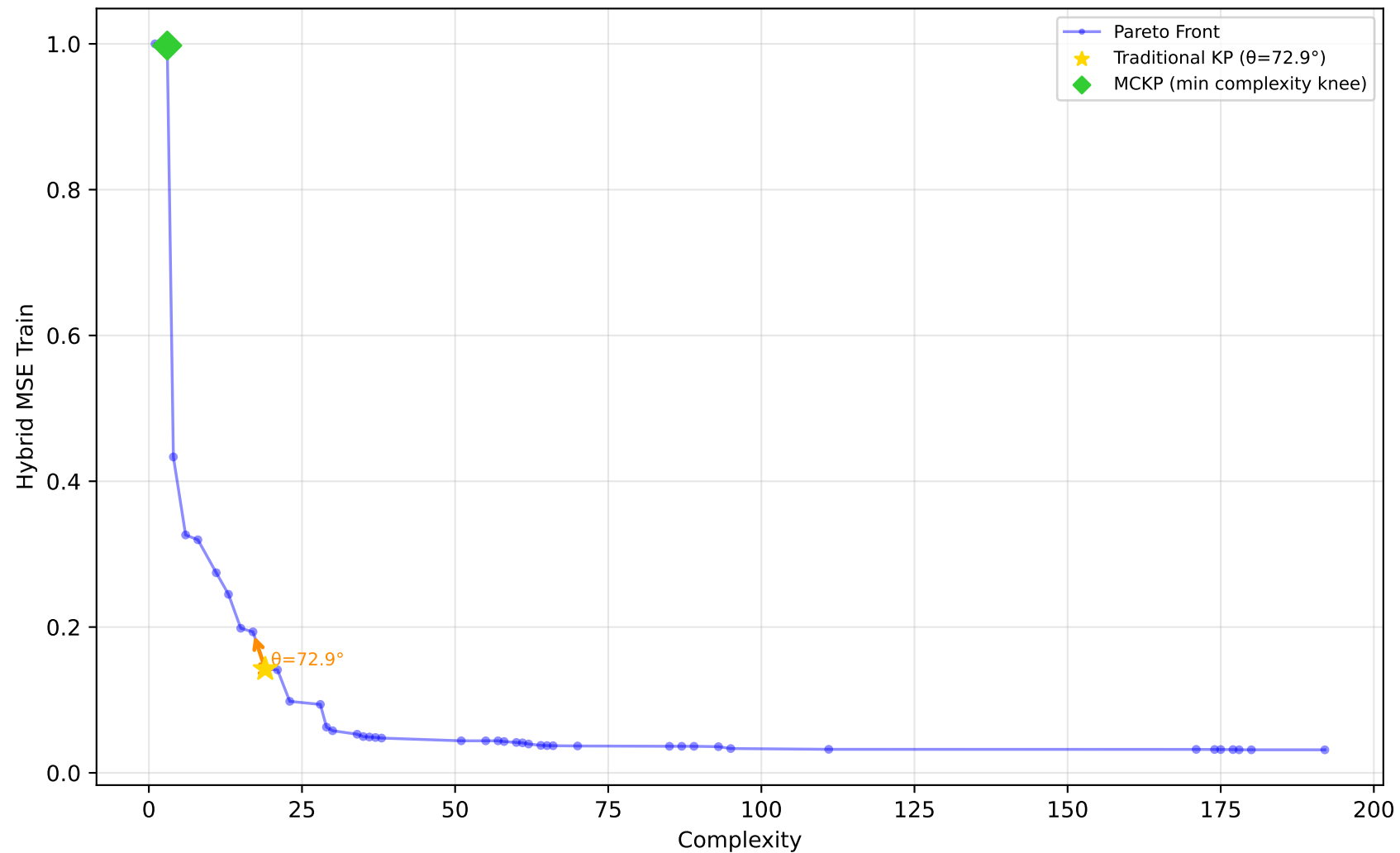
589_fri_c2_1000_25 - Run 12 - MVP - Hybrid MSE Train \lambda_1=0.00, \bar{\lambda}_2=0.00, \bar{\lambda}_3=0.00 | Difficulty: 1.00 | Method: hmr
