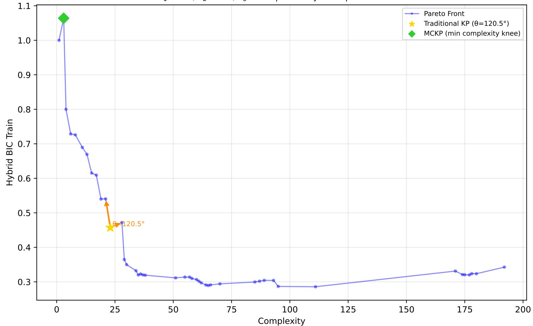
589_fri_c2_1000_25 - Run 12 - SVP - Hybrid BIC Train \lambda_1=0.20 , \bar{\lambda}_2=0.00 , \bar{\lambda}_3=1.00 | Difficulty: 1.00 | Method: hmr
