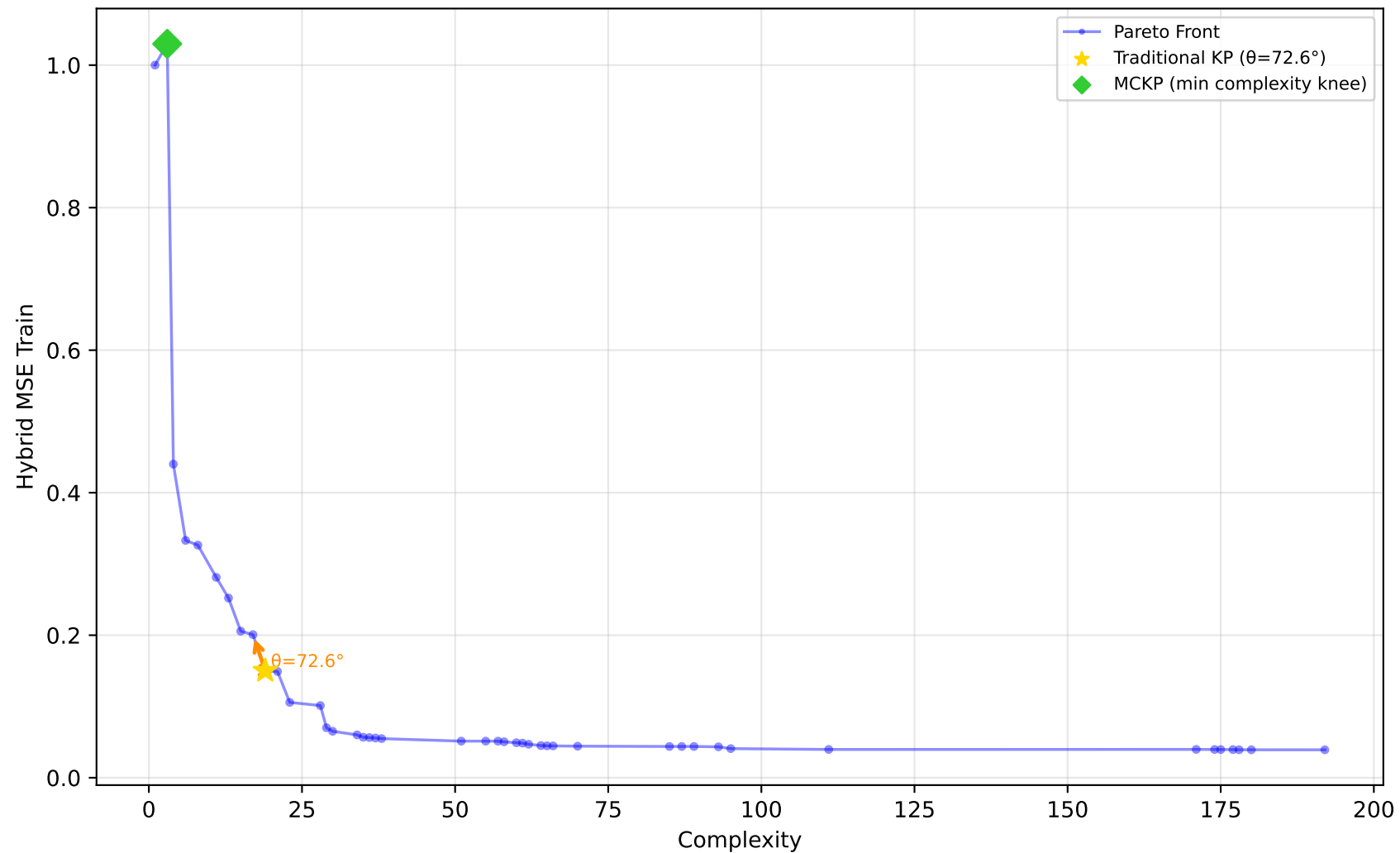
589_fri_c2_1000_25 - Run 12 - SVP - Hybrid MSE Train \lambda_1=0.10, \bar{\lambda}_2=0.00, \bar{\lambda}_3=0.10 | Difficulty: 1.00 | Method: hmr
