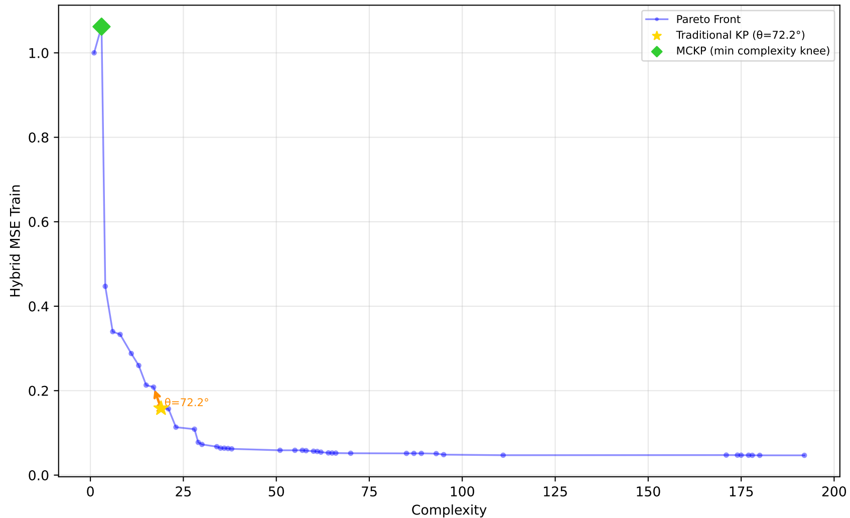
589_fri_c2_1000_25 - Run 12 - SVP - Hybrid MSE Train \lambda_1=0.20, \bar{\lambda}_2=0.00, \bar{\lambda}_3=1.00 | Difficulty: 1.00 | Method: hmr
