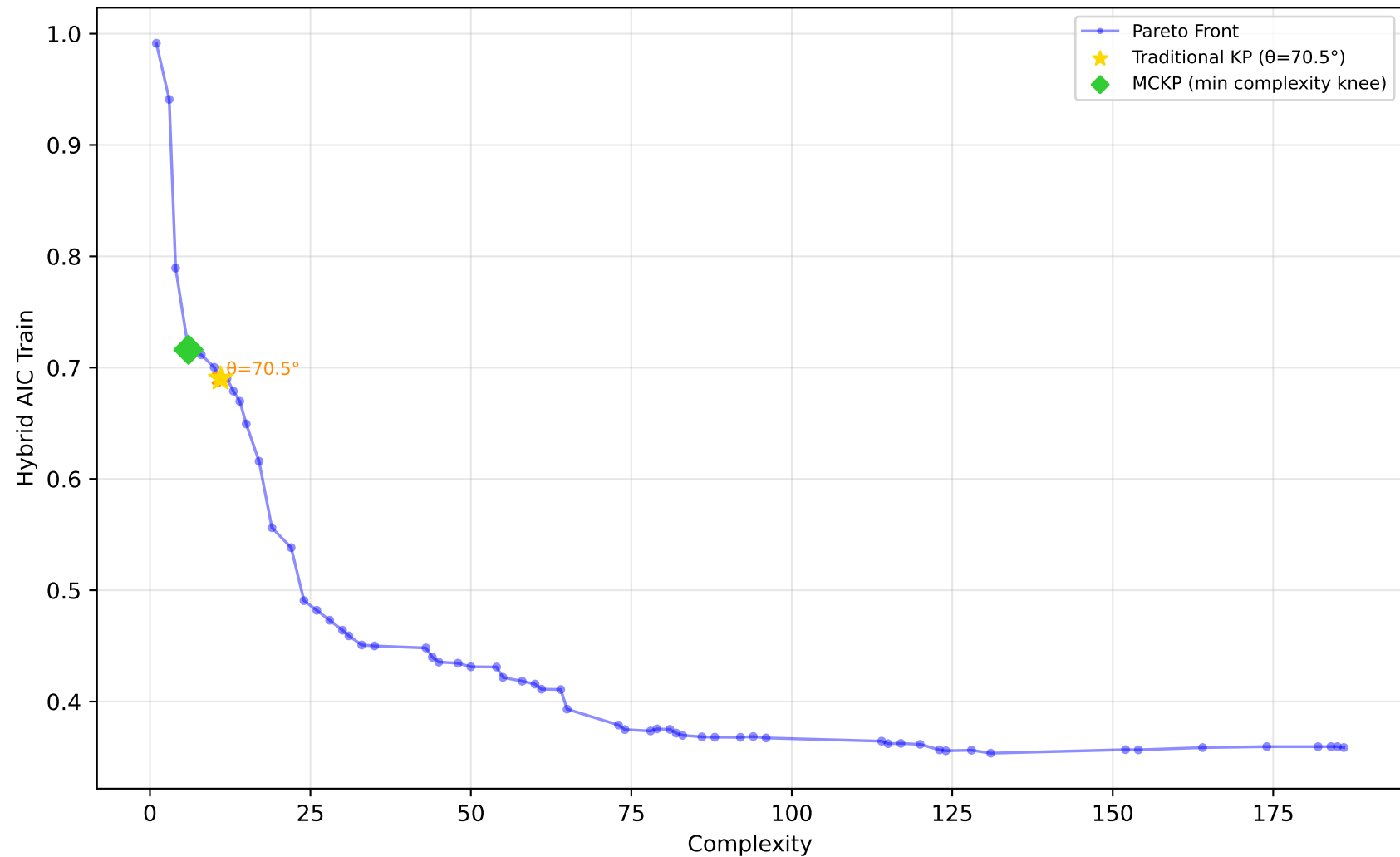
589_fri_c2_1000_25 - Run 13 - MVP - Hybrid AIC Train \lambda_1=0.00, \lambda_2=0.00, \lambda_3=0.00 | Difficulty: 1.00 | Method: hmr
