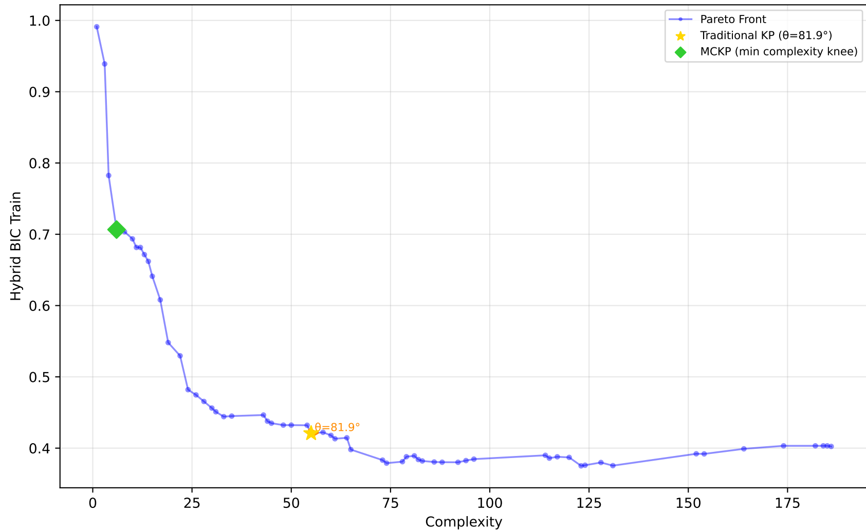
589_fri_c2_1000_25 - Run 13 - MVP - Hybrid BIC Train \lambda_1=0.00, \lambda_2=0.00, \lambda_3=0.00 | Difficulty: 1.00 | Method: hmr
