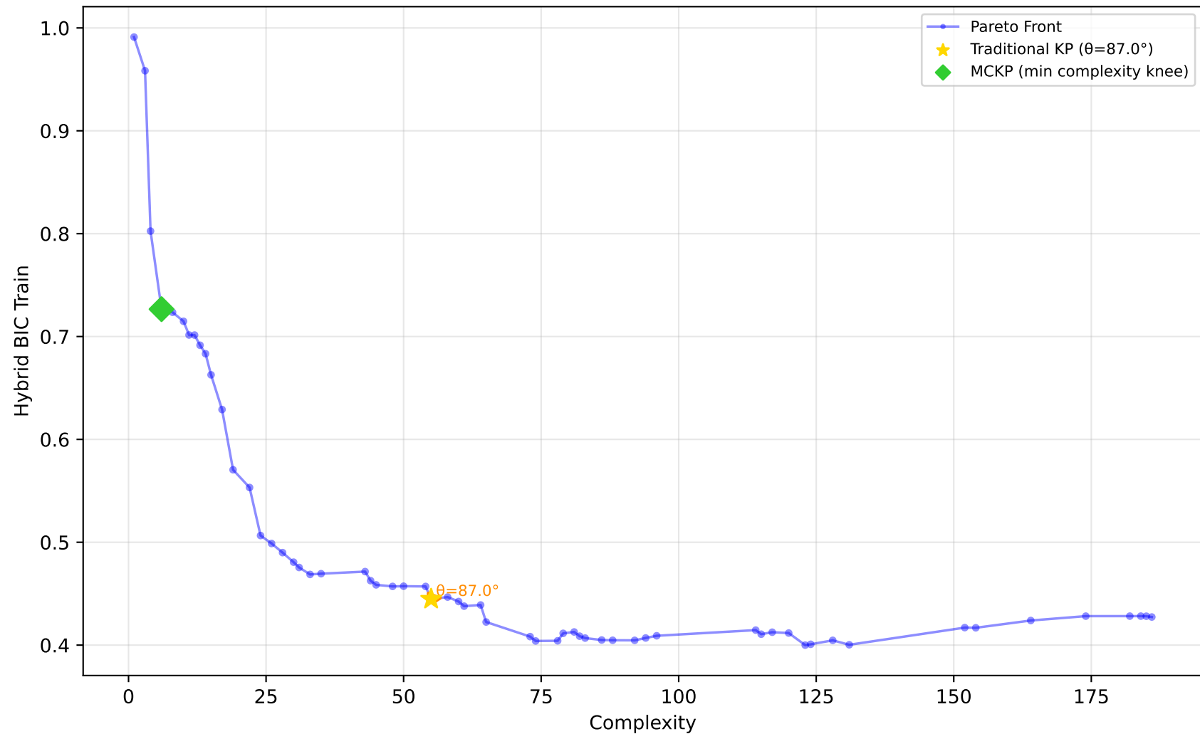
589_fri_c2_1000_25 - Run 13 - MVP - Hybrid BIC Train \lambda_1=0.30, \bar{\lambda}_2=0.00, \bar{\lambda}_3=0.20 | Difficulty: 1.00 | Method: hmr
