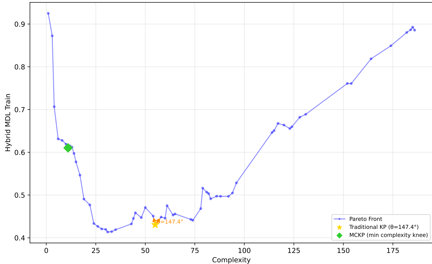
589_fri_c2_1000_25 - Run 13 - MVP - Hybrid MDL Train \lambda_1=0.00, \lambda_2=0.00, \lambda_3=0.00 | Difficulty: 1.00 | Method: hmr
