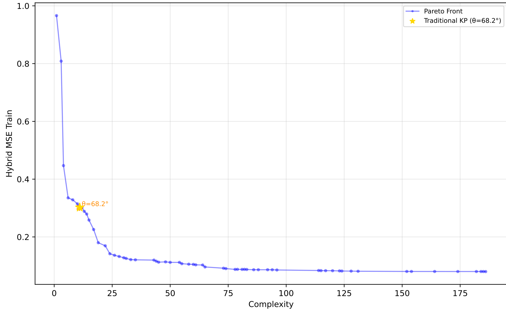
589_fri_c2_1000_25 - Run 13 - MVP - Hybrid MSE Train \lambda_1=0.30, \lambda_2=0.00, \lambda_3=0.20 | Difficulty: 1.00 | Method: hmr
