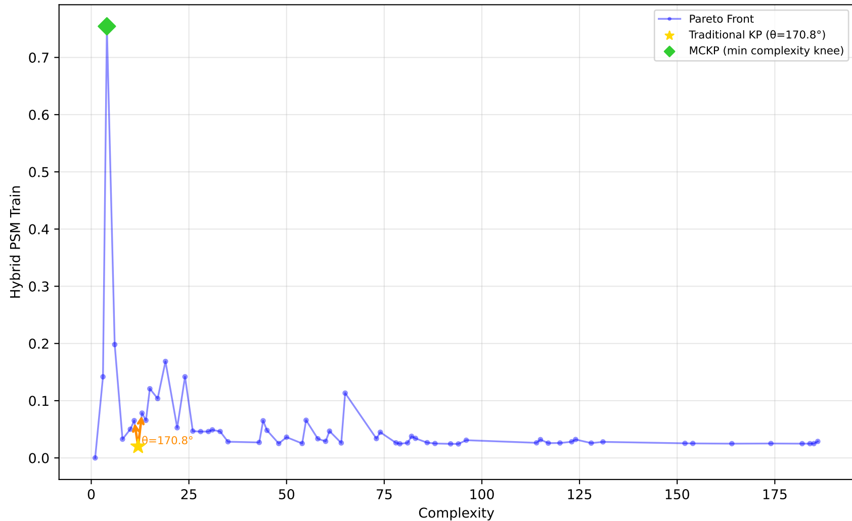
589_fri_c2_1000_25 - Run 13 - MVP - Hybrid PSM Train \lambda_1=0.30, \lambda_2=0.00, \lambda_3=0.20 | Difficulty: 1.00 | Method: hmr
