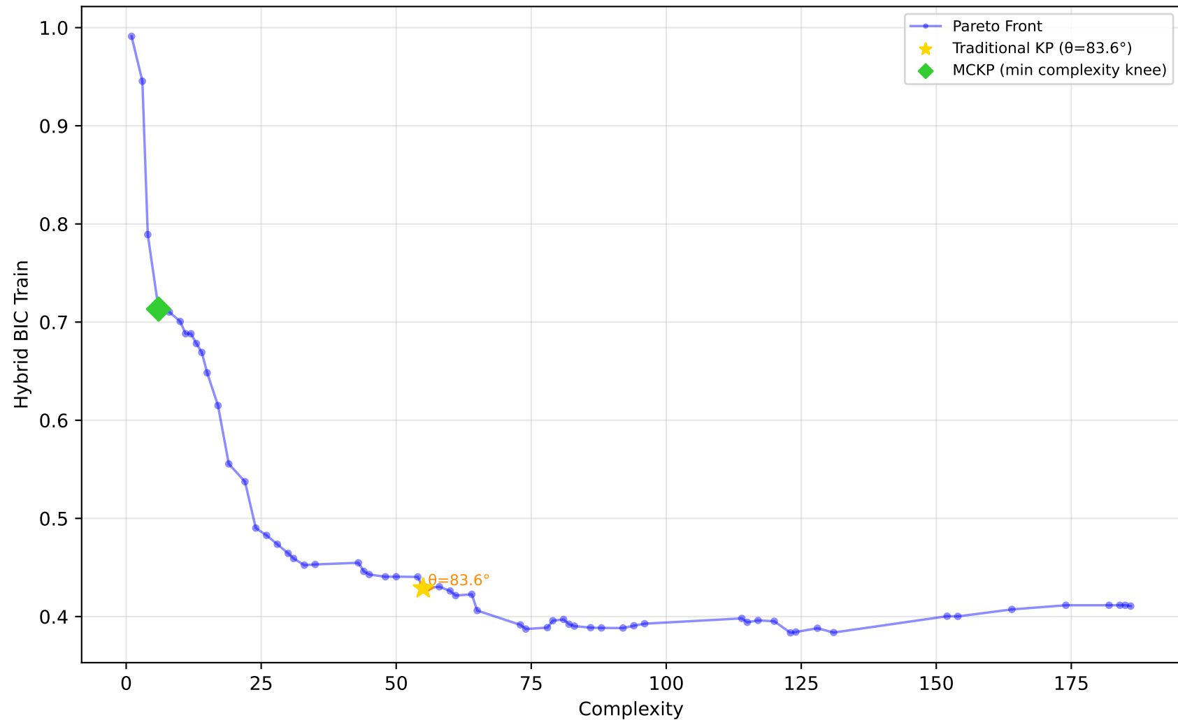
589_fri_c2_1000_25 - Run 13 - SVP - Hybrid BIC Train \lambda_1=0.10, \bar{\lambda}_2=0.00, \bar{\lambda}_3=0.10 | Difficulty: 1.00 | Method: hmr
