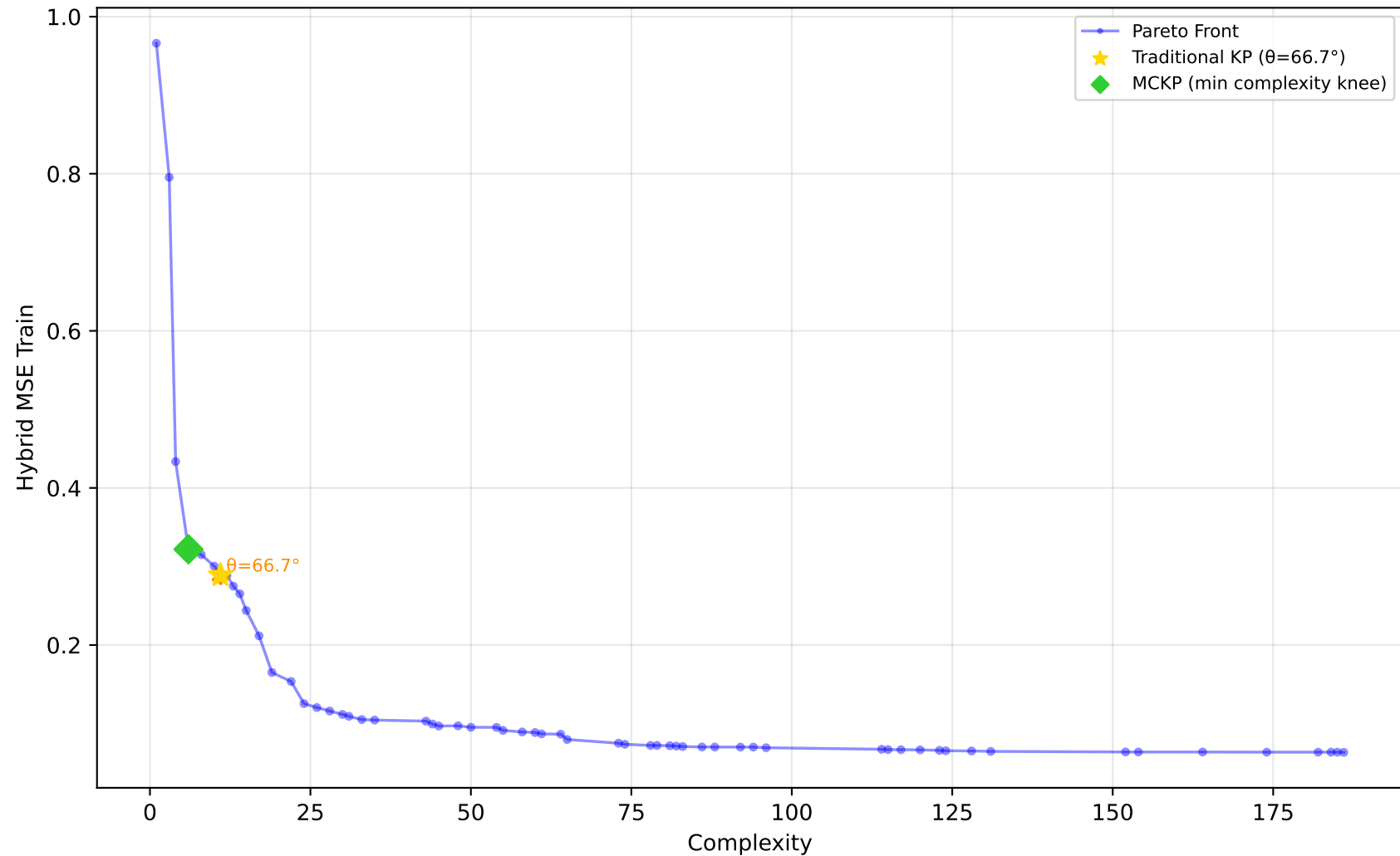
589_fri_c2_1000_25 - Run 13 - SVP - Hybrid MSE Train \lambda_1=0.10, \bar{\lambda}_2=0.00, \bar{\lambda}_3=0.10 | Difficulty: 1.00 | Method: hmr
