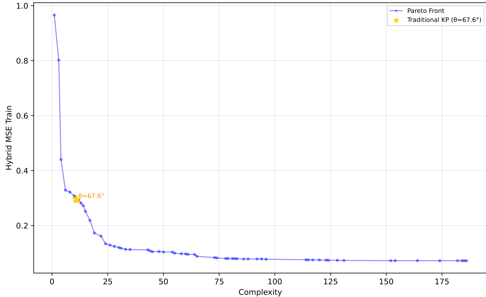
589_fri_c2_1000_25 - Run 13 - SVP - Hybrid MSE Train \lambda_1=0.20 , \lambda_2=0.00 , \lambda_3=1.00 | Difficulty: 1.00 | Method: hmr
