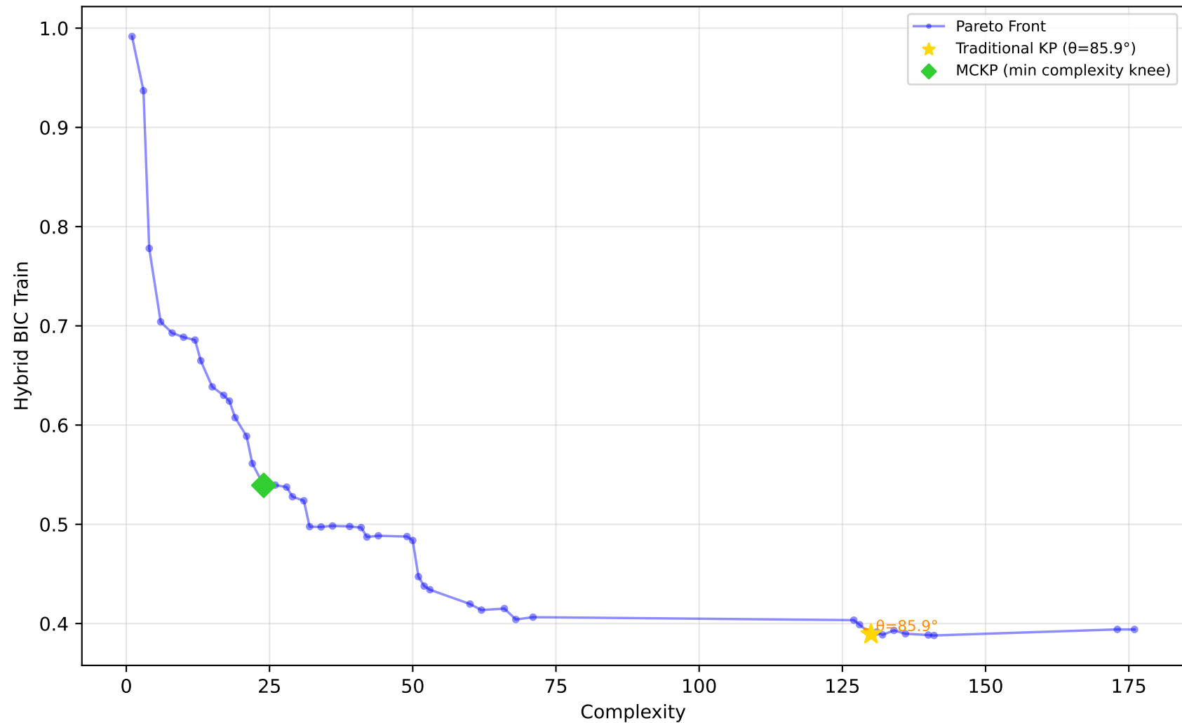
589_fri_c2_1000_25 - Run 14 - MVP - Hybrid BIC Train \lambda_1=0.00, \bar{\lambda}_2=0.00, \bar{\lambda}_3=0.00 | Difficulty: 1.00 | Method: hmr
