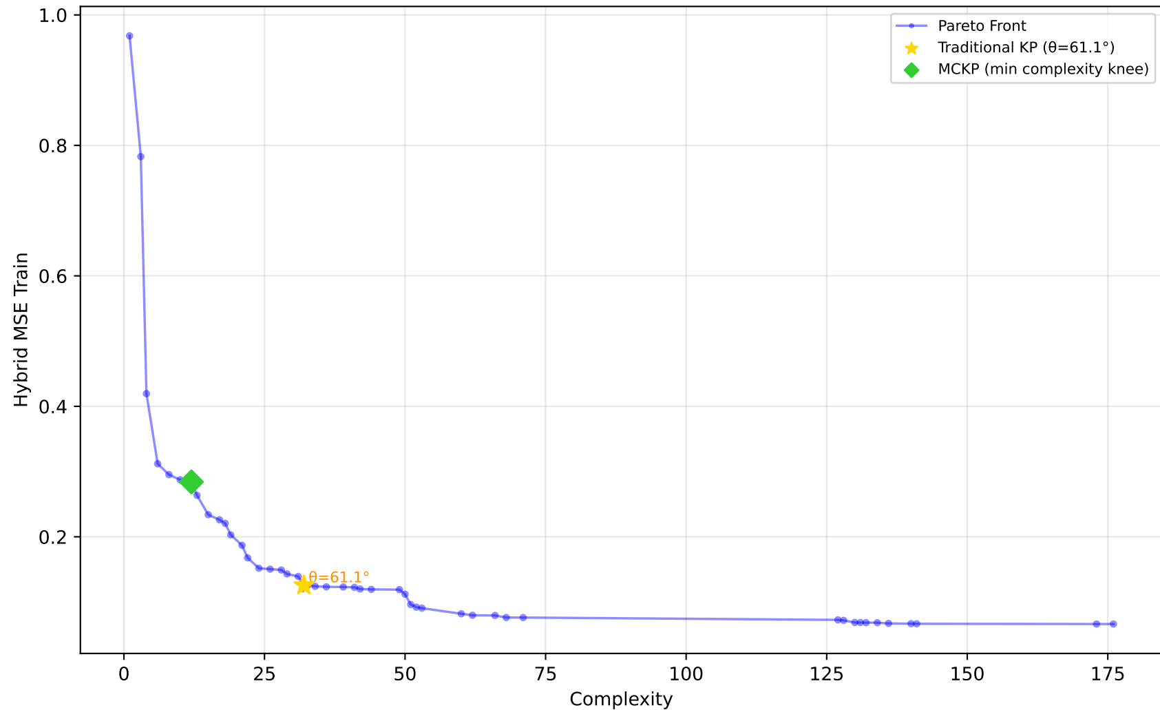
589_fri_c2_1000_25 - Run 14 - MVP - Hybrid MSE Train \lambda_1=0.00, \lambda_2=0.00, \lambda_3=0.00 | Difficulty: 1.00 | Method: hmr
