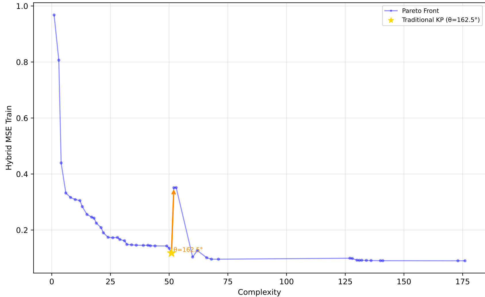
589_fri_c2_1000_25 - Run 14 - MVP - Hybrid MSE Train \lambda_1=0.30, \lambda_2=0.00, \lambda_3=0.20 | Difficulty: 1.00 | Method: hmr
