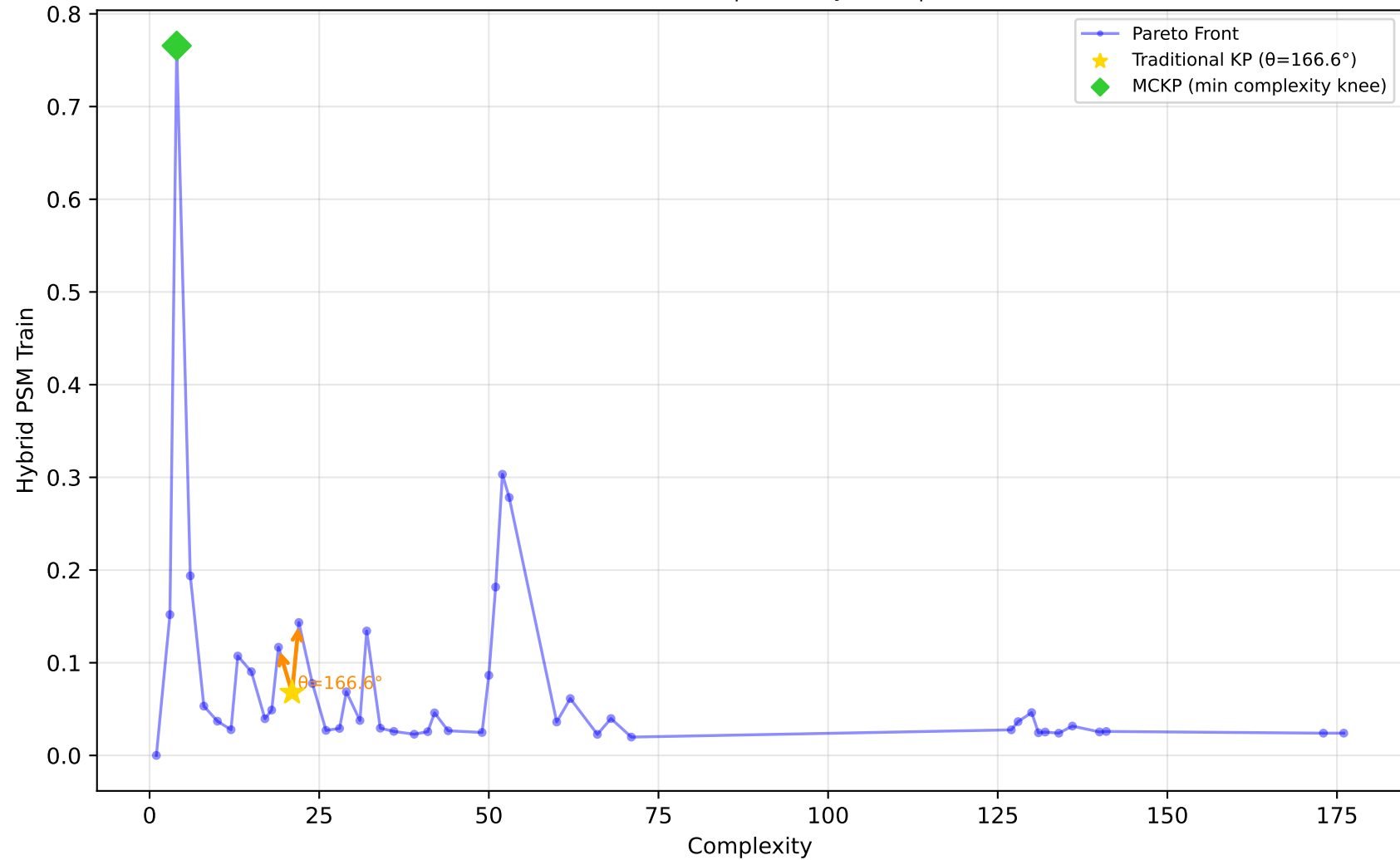
589_fri_c2_1000_25 - Run 14 - MVP - Hybrid PSM Train \lambda_1=0.30, \lambda_2=0.00, \lambda_3=0.20 | Difficulty: 1.00 | Method: hmr
