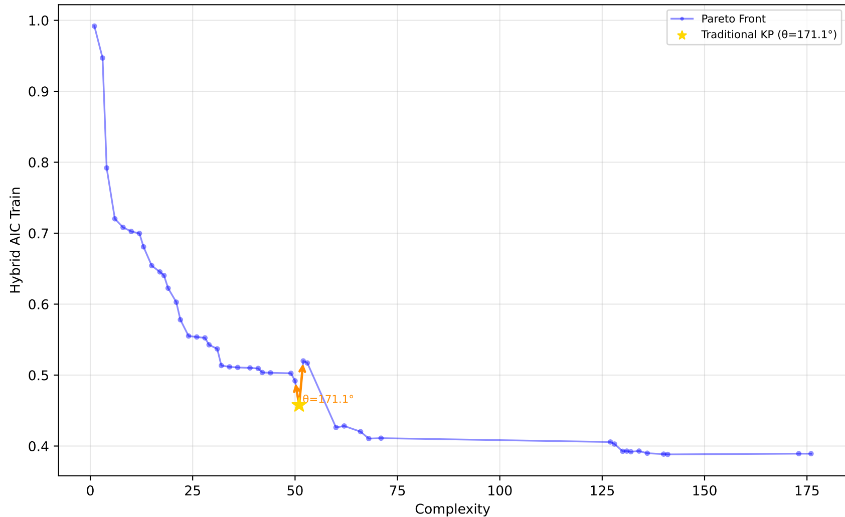
589_fri_c2_1000_25 - Run 14 - SVP - Hybrid AIC Train \lambda_1=0.10, \bar{\lambda}_2=0.00, \bar{\lambda}_3=0.10 | Difficulty: 1.00 | Method: hmr
