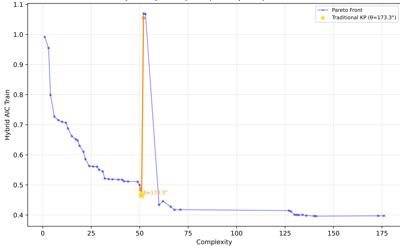
589_fri_c2_1000_25 - Run 14 - SVP - Hybrid AIC Train \lambda_1=0.20 , \lambda_2=0.00 , \lambda_3=1.00 | Difficulty: 1.00 | Method: hmr
