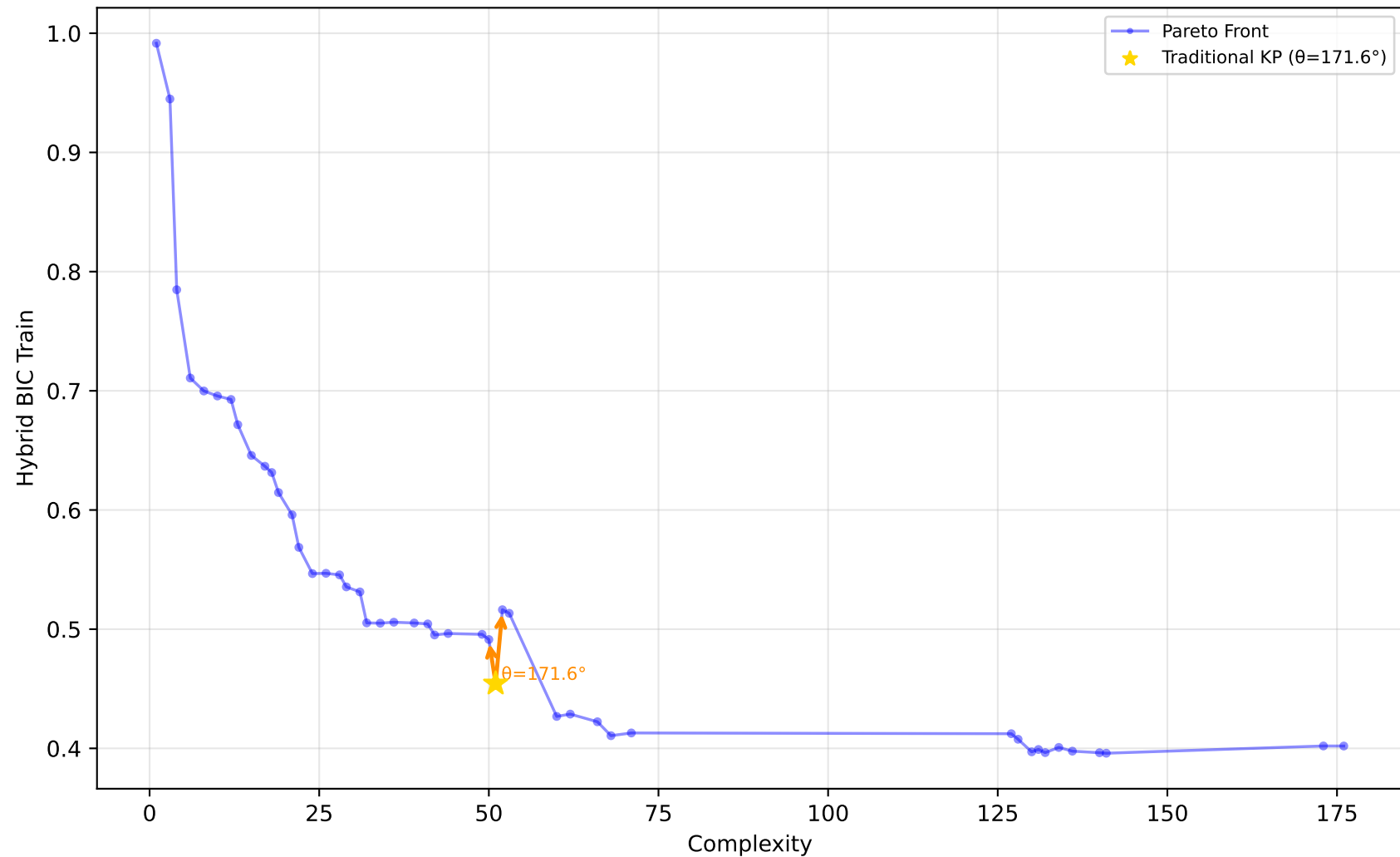
589_fri_c2_1000_25 - Run 14 - SVP - Hybrid BIC Train \lambda_1=0.10, \bar{\lambda}_2=0.00, \bar{\lambda}_3=0.10 | Difficulty: 1.00 | Method: hmr
