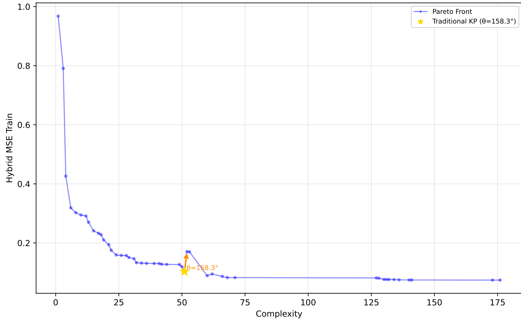
589_fri_c2_1000_25 - Run 14 - SVP - Hybrid MSE Train \lambda_1=0.10, \bar{\lambda}_2=0.00, \bar{\lambda}_3=0.10 | Difficulty: 1.00 | Method: hmr
