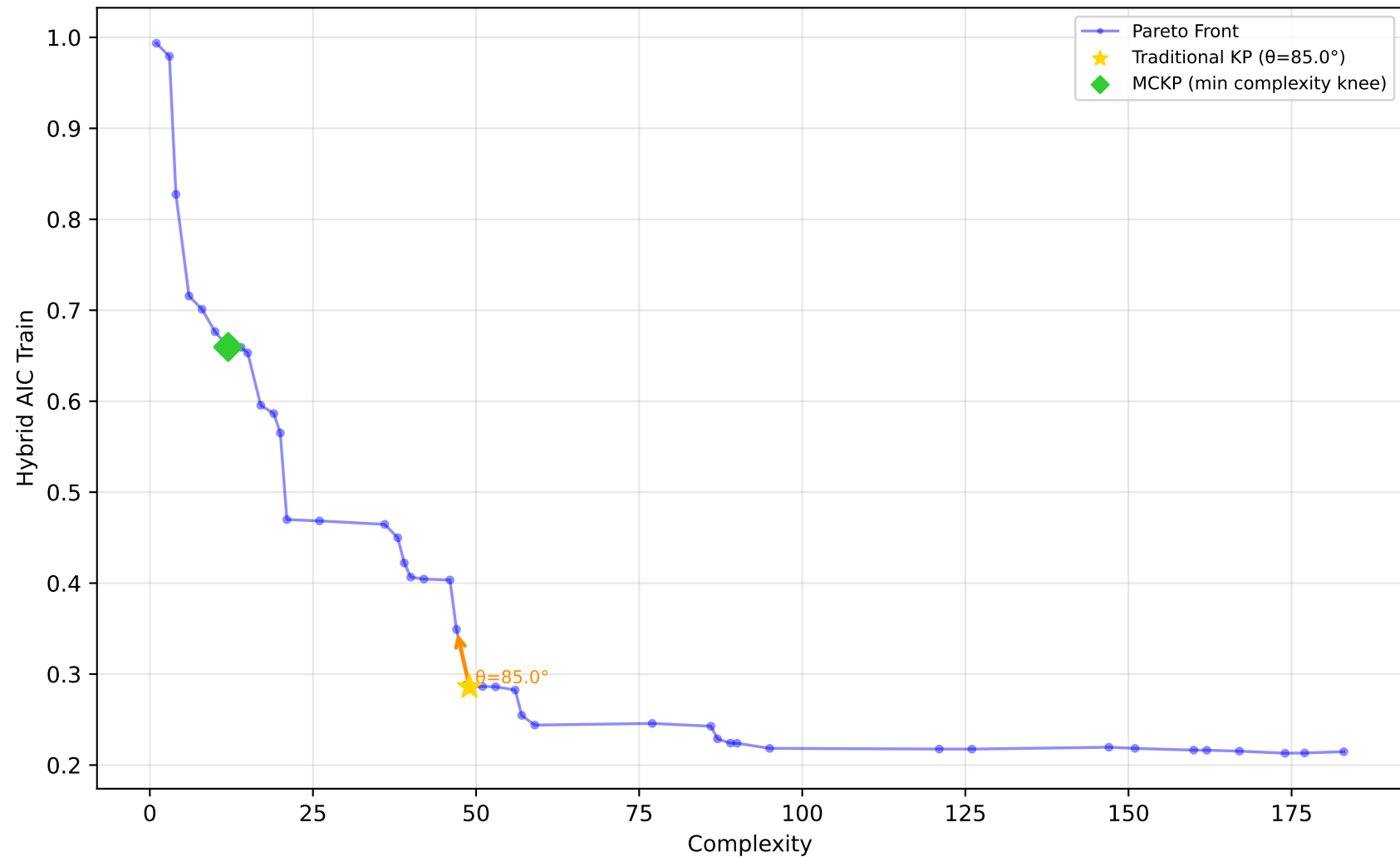
589_fri_c2_1000_25 - Run 15 - MVP - Hybrid AIC Train \lambda_1=0.00, \bar{\lambda}_2=0.00, \bar{\lambda}_3=0.00 | Difficulty: 1.00 | Method: hmr
