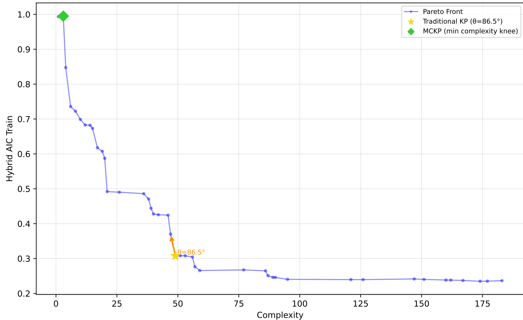
589_fri_c2_1000_25 - Run 15 - MVP - Hybrid AIC Train \lambda_1=0.30, \bar{\lambda}_2=0.00, \bar{\lambda}_3=0.20 | Difficulty: 1.00 | Method: hmr
