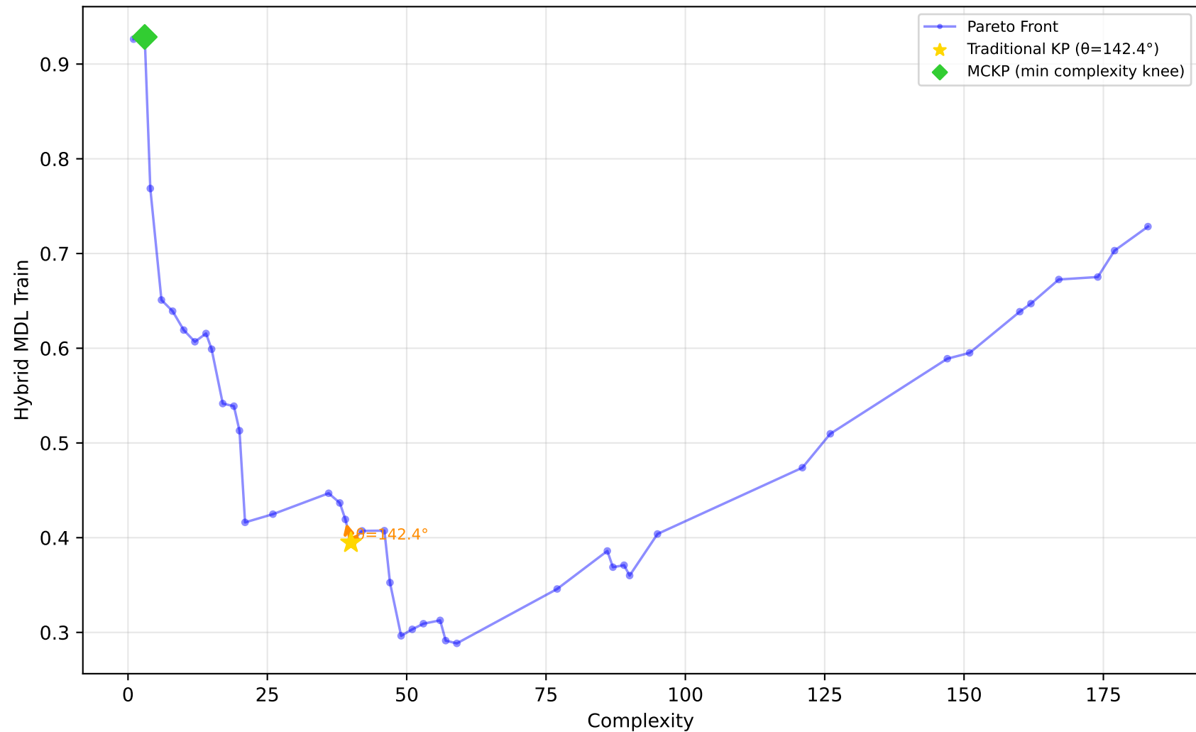
589_fri_c2_1000_25 - Run 15 - MVP - Hybrid MDL Train \lambda_1=0.30, \lambda_2=0.00, \lambda_3=0.20 | Difficulty: 1.00 | Method: hmr
