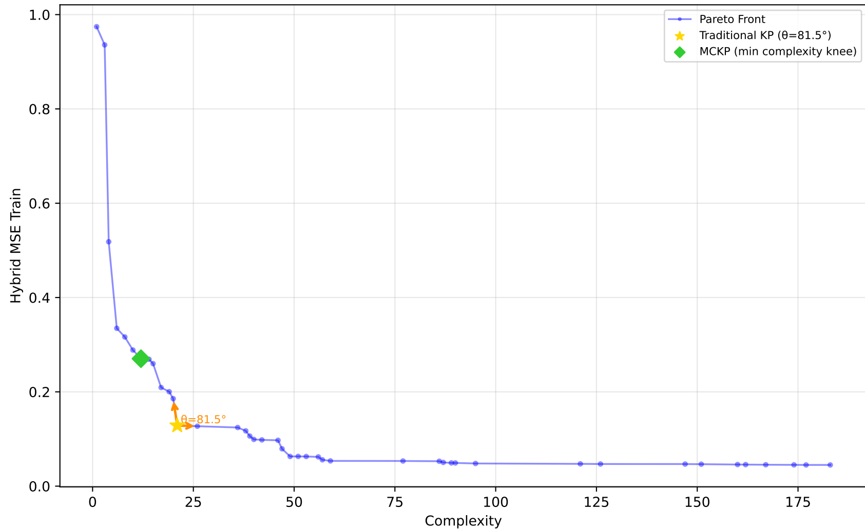
589_fri_c2_1000_25 - Run 15 - MVP - Hybrid MSE Train \lambda_1=0.30, \lambda_2=0.00, \lambda_3=0.20 | Difficulty: 1.00 | Method: hmr
