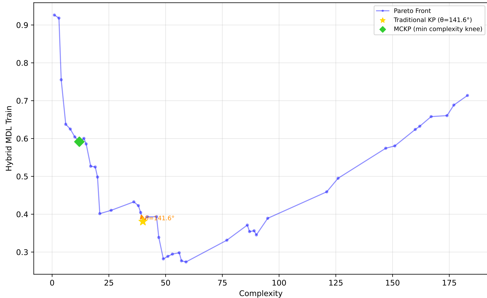
589_fri_c2_1000_25 - Run 15 - SVP - Hybrid MDL Train \lambda_1=0.10, \bar{\lambda}_2=0.00, \bar{\lambda}_3=0.10 | Difficulty: 1.00 | Method: hmr
