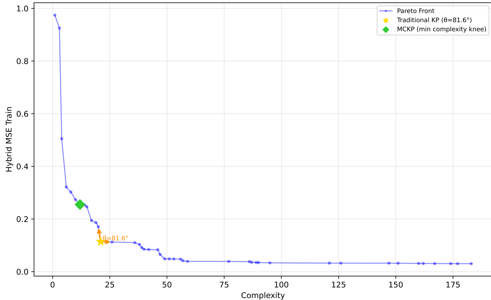
589_fri_c2_1000_25 - Run 15 - SVP - Hybrid MSE Train \lambda_1=0.10, \bar{\lambda}_2=0.00, \bar{\lambda}_3=0.10 | Difficulty: 1.00 | Method: hmr
