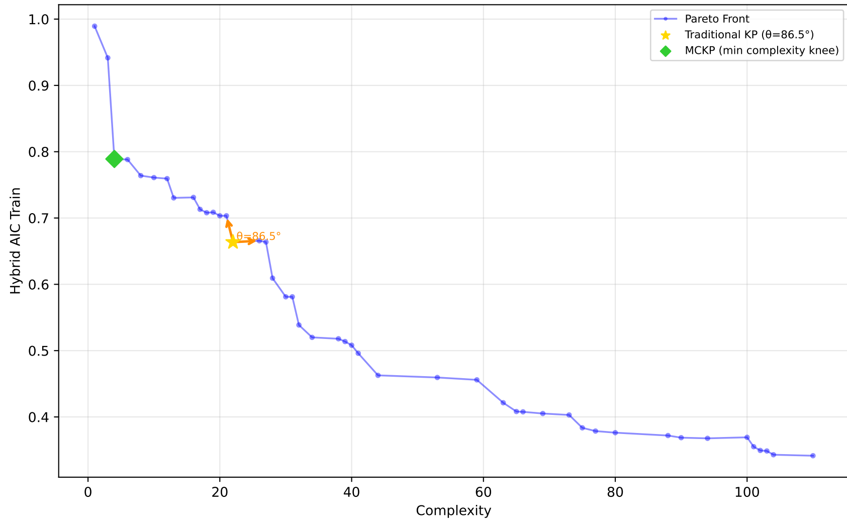
589_fri_c2_1000_25 - Run 16 - MVP - Hybrid AIC Train \lambda_1=0.00, \lambda_2=0.00, \lambda_3=0.00 | Difficulty: 1.00 | Method: hmr
