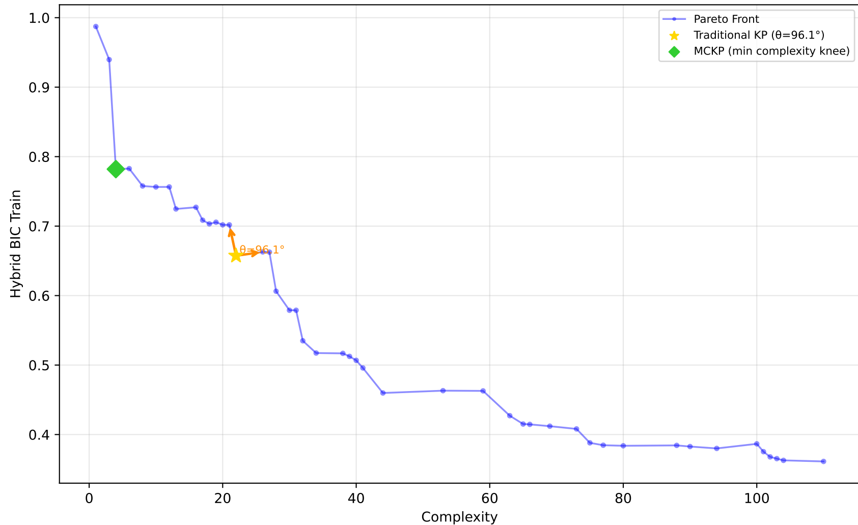
589_fri_c2_1000_25 - Run 16 - MVP - Hybrid BIC Train \lambda_1=0.00, \lambda_2=0.00, \lambda_3=0.00 | Difficulty: 1.00 | Method: hmr
