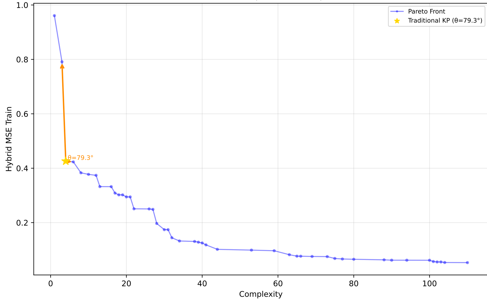
589_fri_c2_1000_25 - Run 16 - MVP - Hybrid MSE Train \lambda_1=0.00, \lambda_2=0.00, \lambda_3=0.00 | Difficulty: 1.00 | Method: hmr
