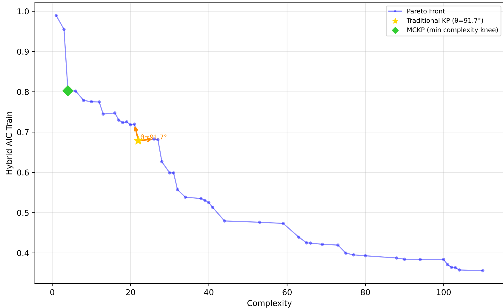
589_fri_c2_1000_25 - Run 16 - SVP - Hybrid AIC Train \lambda_1=0.20, \lambda_2=0.00, \lambda_3=1.00 | Difficulty: 1.00 | Method: hmr
